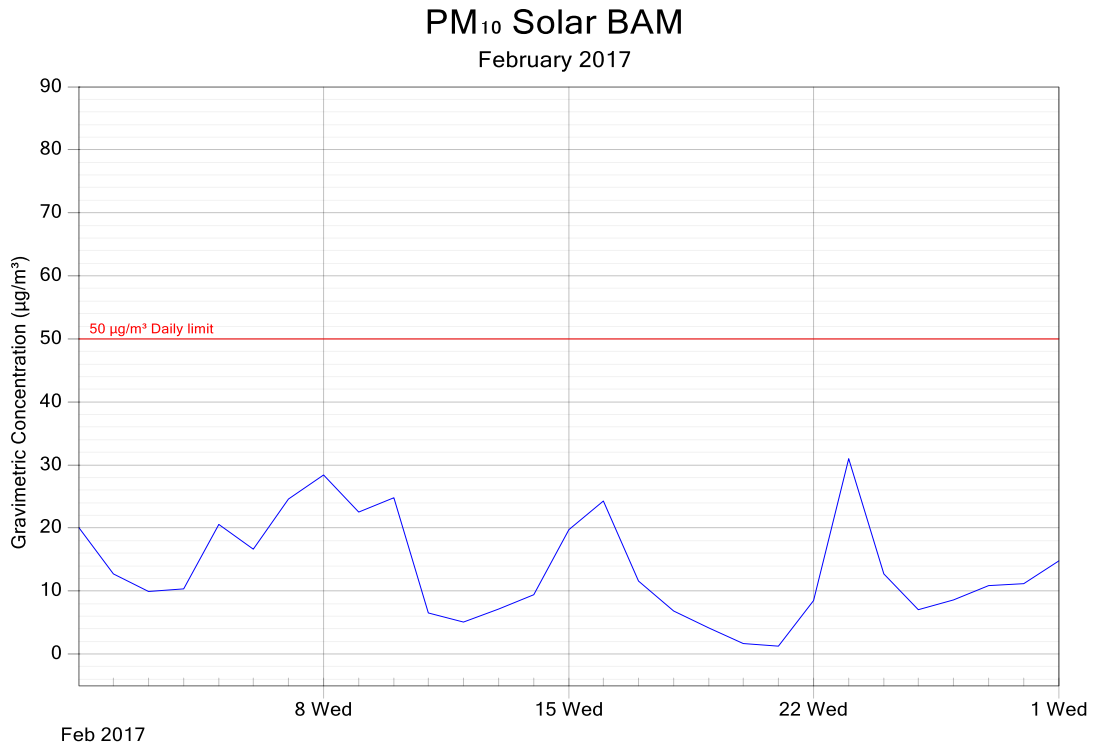
Figure 4: PM 10 for McEwens Beach station 24-hour Averages – February 2017
