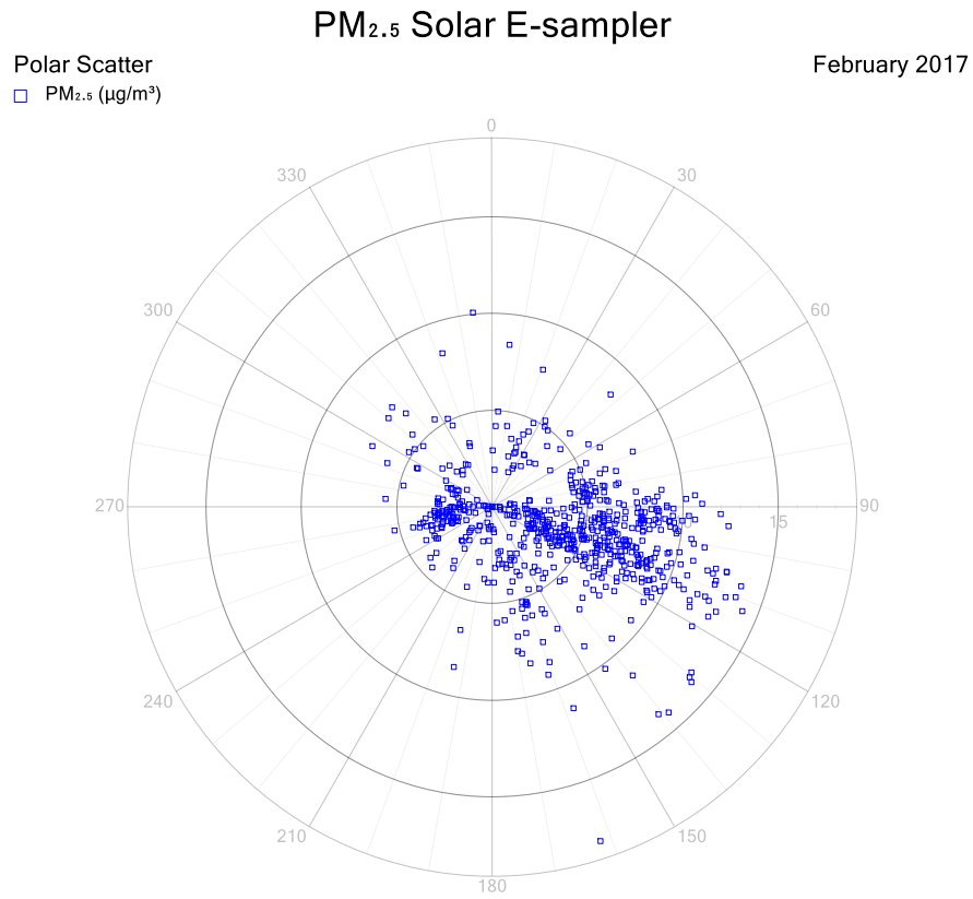
Figure 5: PM 2.5 polar scatter plot (1-hour average) for McEwens Beach station – Feb 2017
