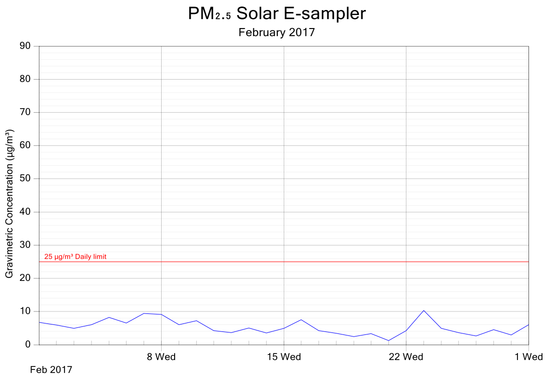
Figure 6: PM 2.5 for McEwens Beach station 24-hour Averages – Feb 2017
