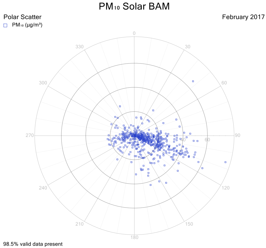
Figure 3: PM 10 polar scatter plot (1-hour average) for McEwens Beach station – Feb 2017
