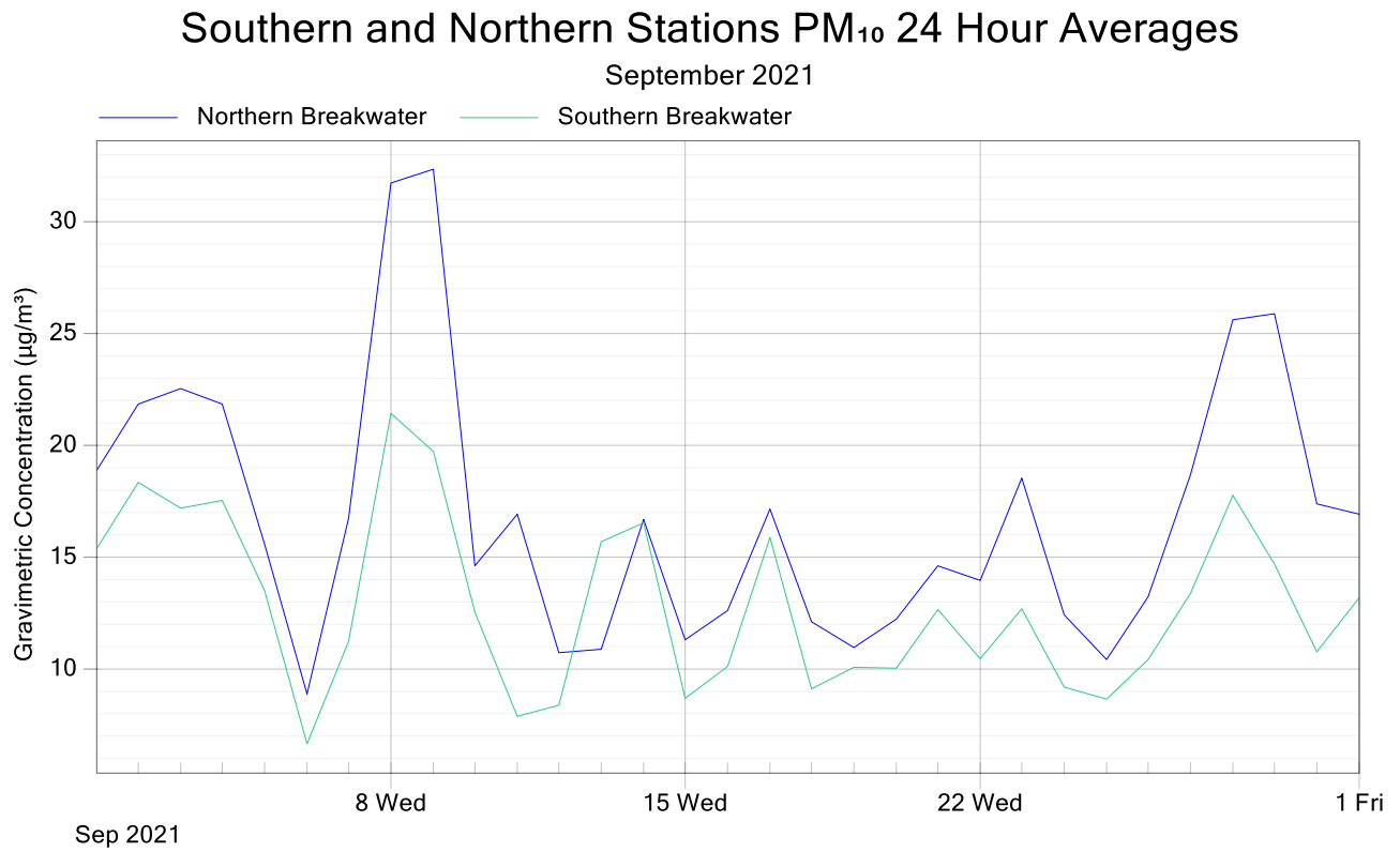
Figure 6: Southern and Northern Stations PM 10 24 Hour Averages Comparison September 2021
