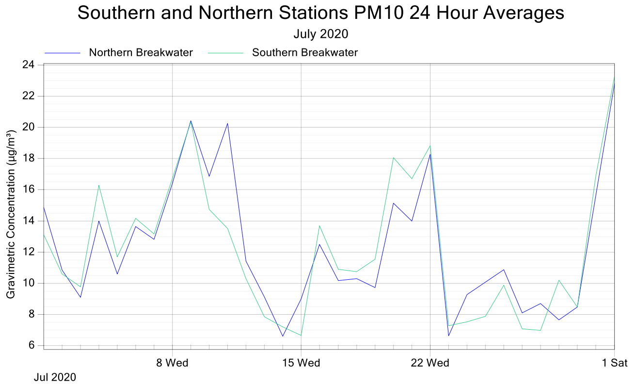
Figure 6: Southern and Northern Stations PM 10 24 Hour Averages Comparison July 2020
