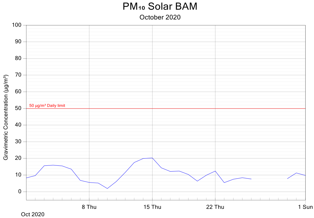
Figure 2: PM 10 for McEwens Beach station 24-hour Averages – October 2020
