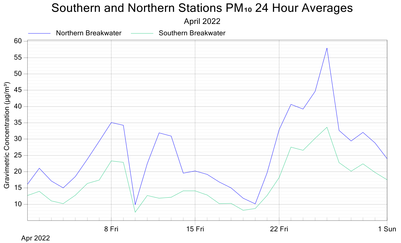
Figure 6: Southern and Northern Stations PM 10 24 Hour Averages Comparison April 2022
