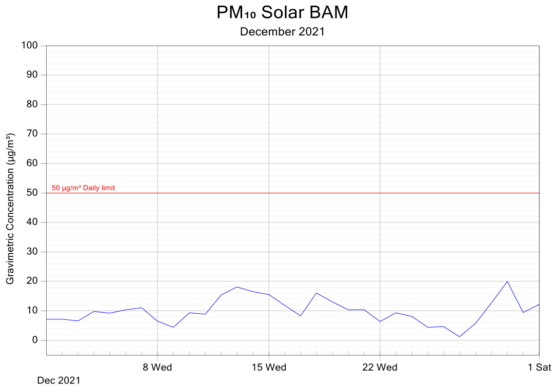
Figure 2: PM 10 for McEwens Beach station 24-hour Averages – December 2021
