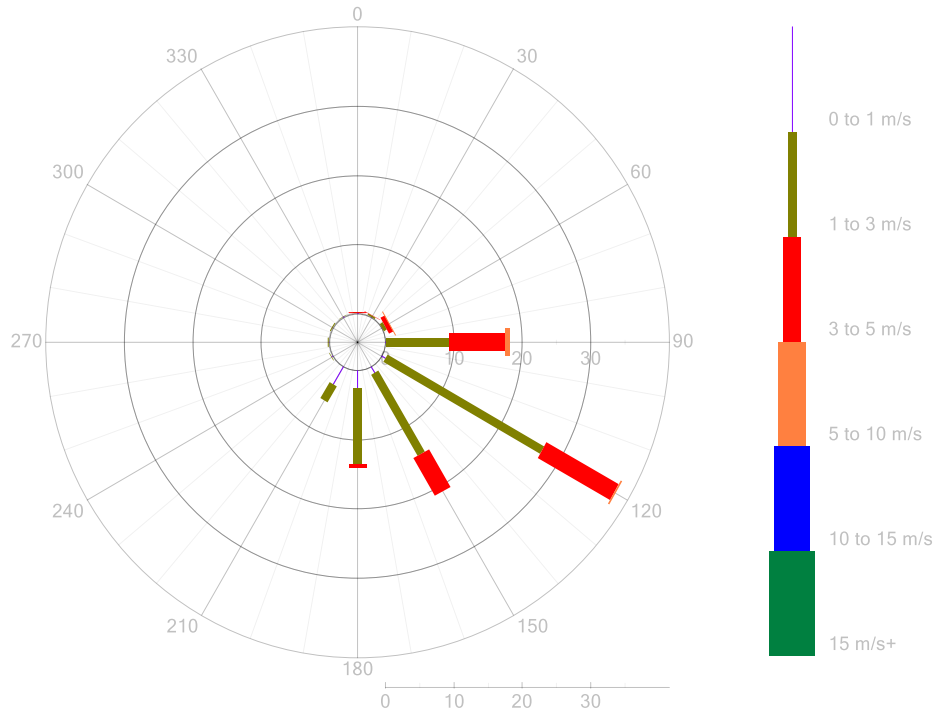
Figure 11: P1 Wind Rose 5-Minute Data for April 2022
