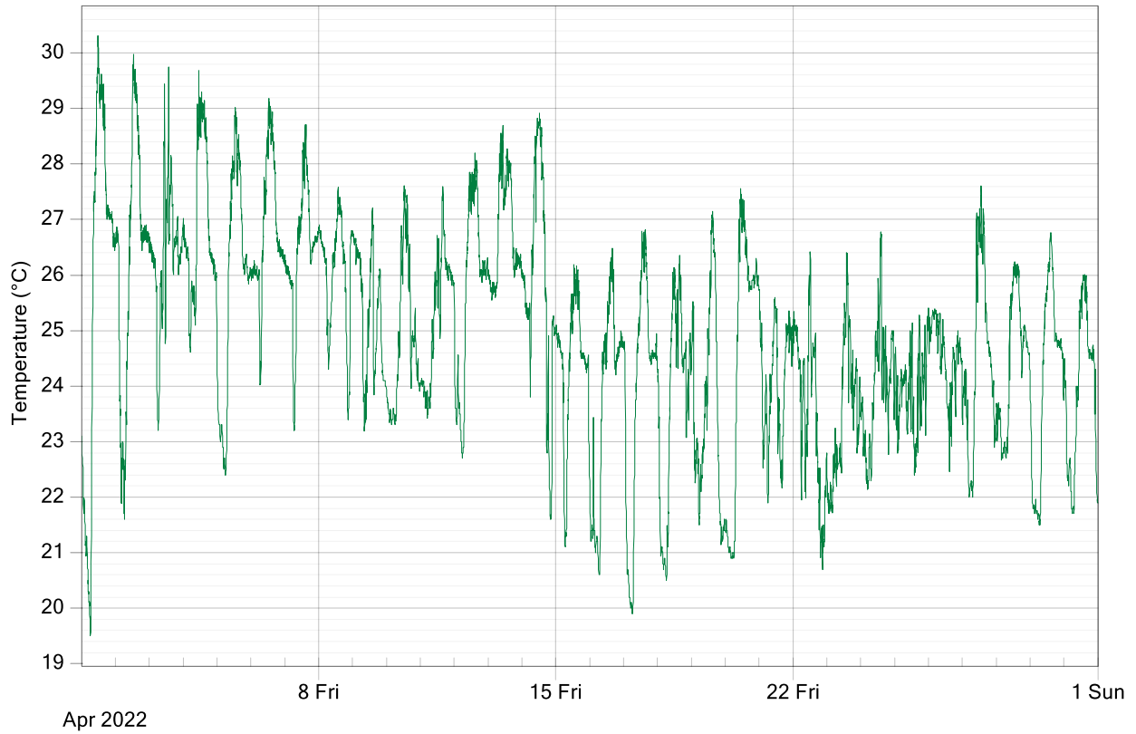
Figure 15: Port of Hay Point AT 5-Minute Averages Data for April 2022
