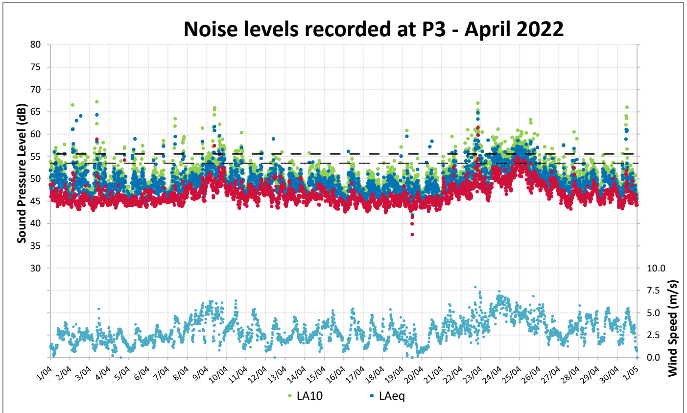
Figure 9: Noise Levels Recorded at P3 for April 2022
