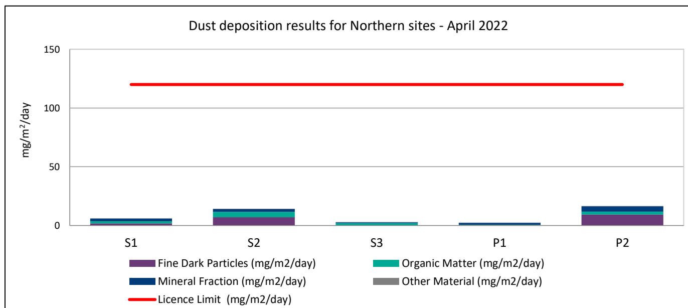
Figure 5: Dust Deposition Results for Northern Sites, April 2022
