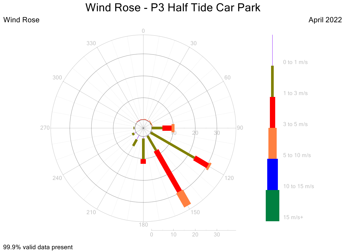
Figure 13: P3 Wind Rose 5-Minute Data for April 2022
