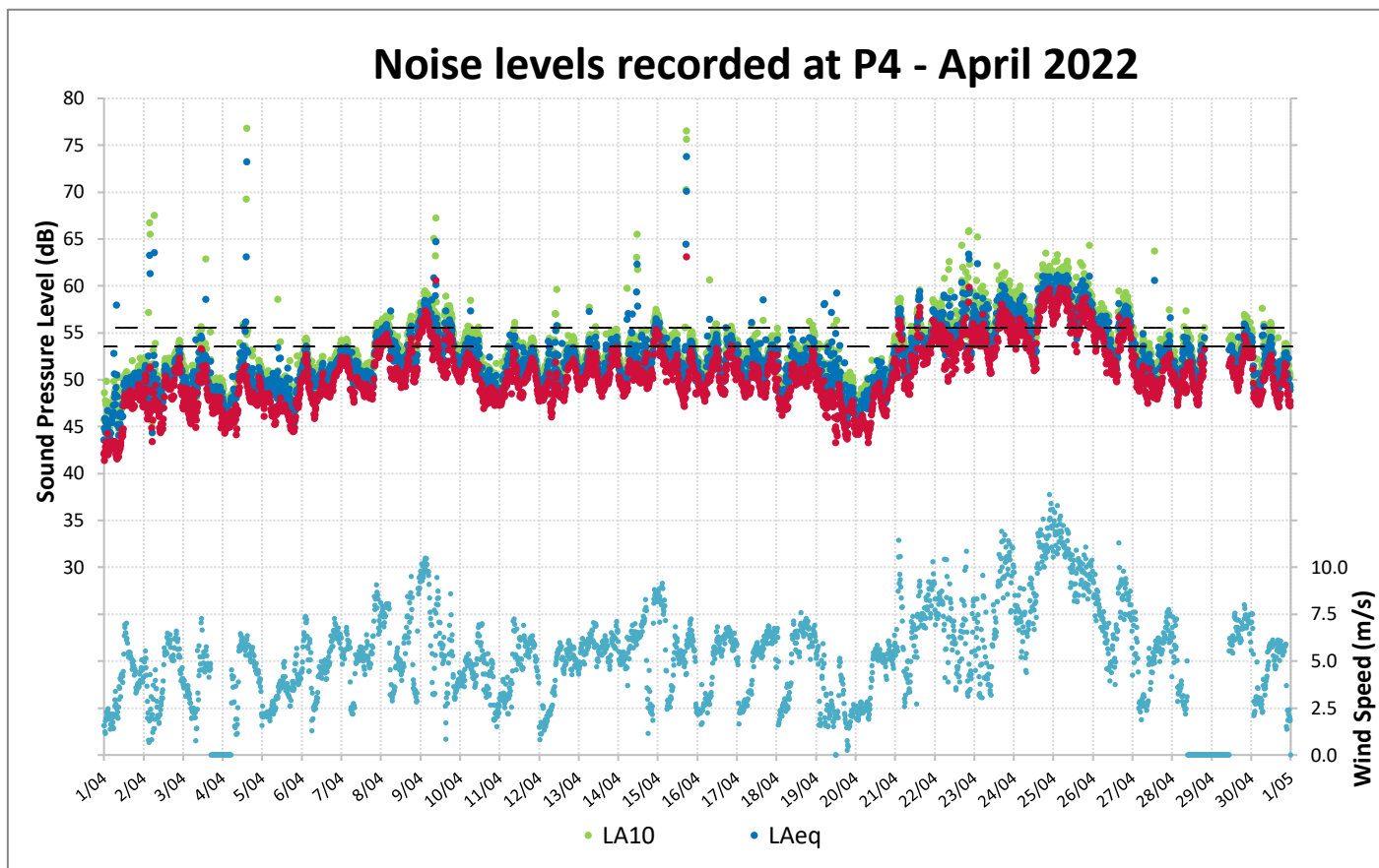
Figure 10: Noise Levels Recorded at P4 for April 2022
