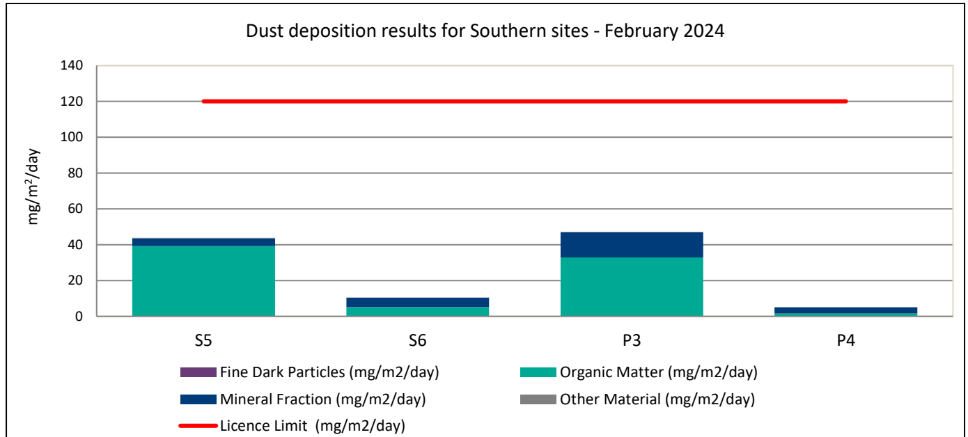
Figure 6: Dust Deposition Results for Southern Sites, February 2024
