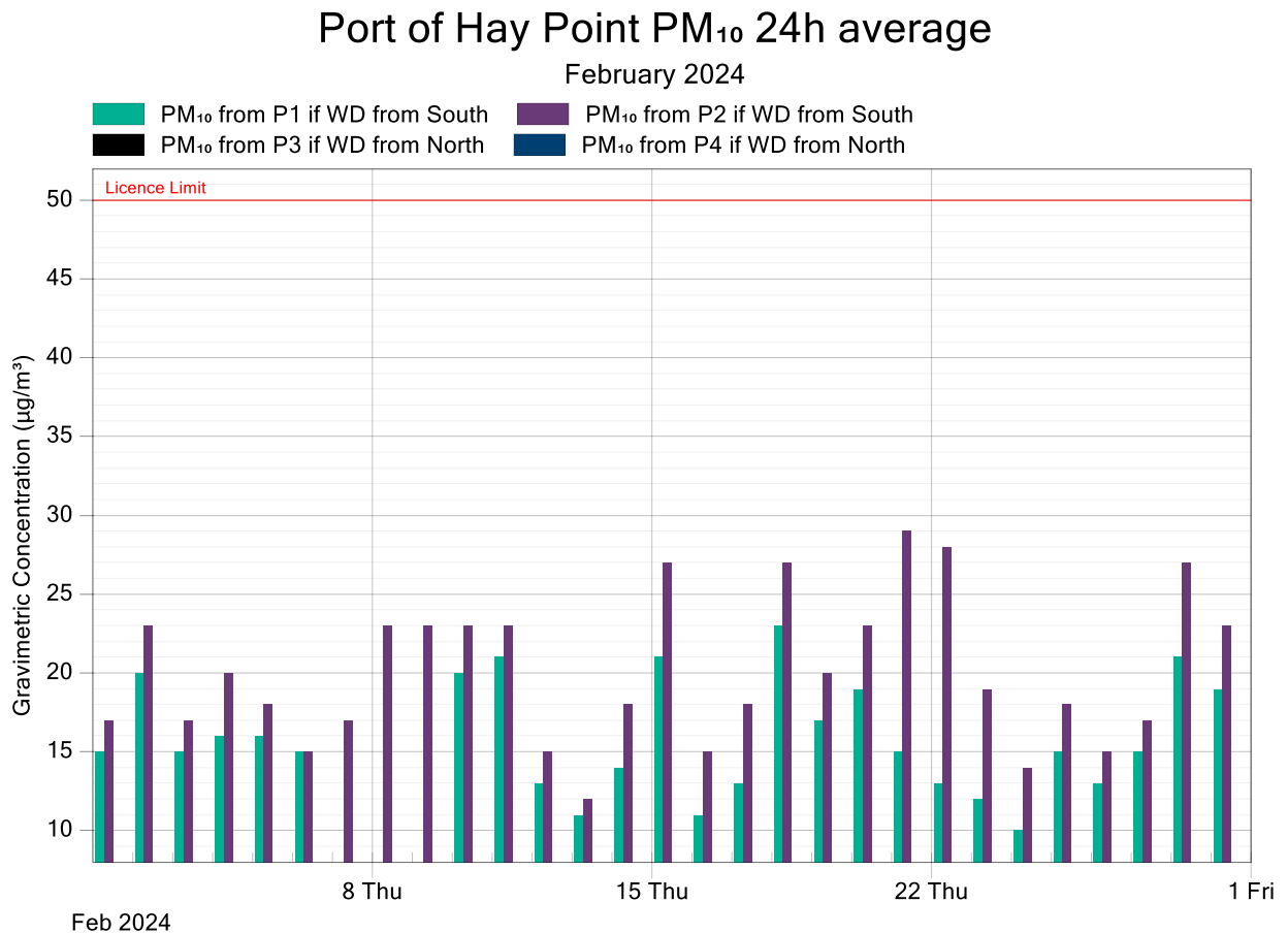
Figure 4: Port of Hay Point PM 10 24-Hour Average Data Compared to the Licence Limit for February 2024
