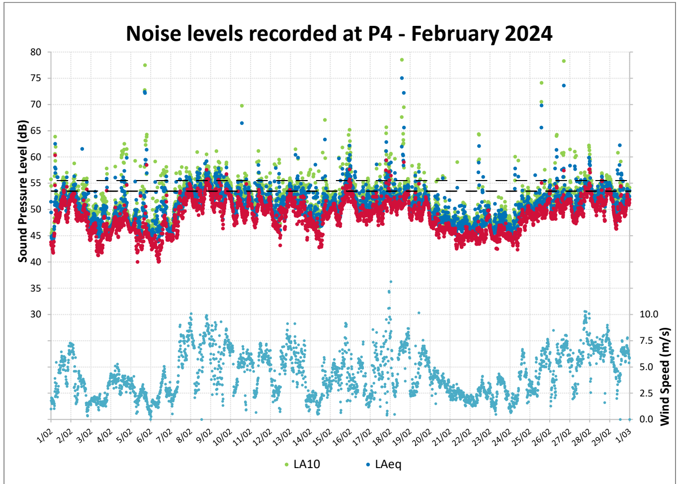
Figure 10: Noise Levels Recorded at P4 for February 2024
