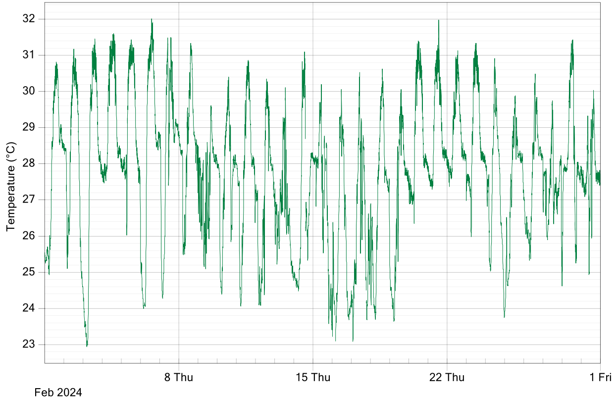
Figure 15: Port of Hay Point AT 5-Minute Averages Data for February 2024
