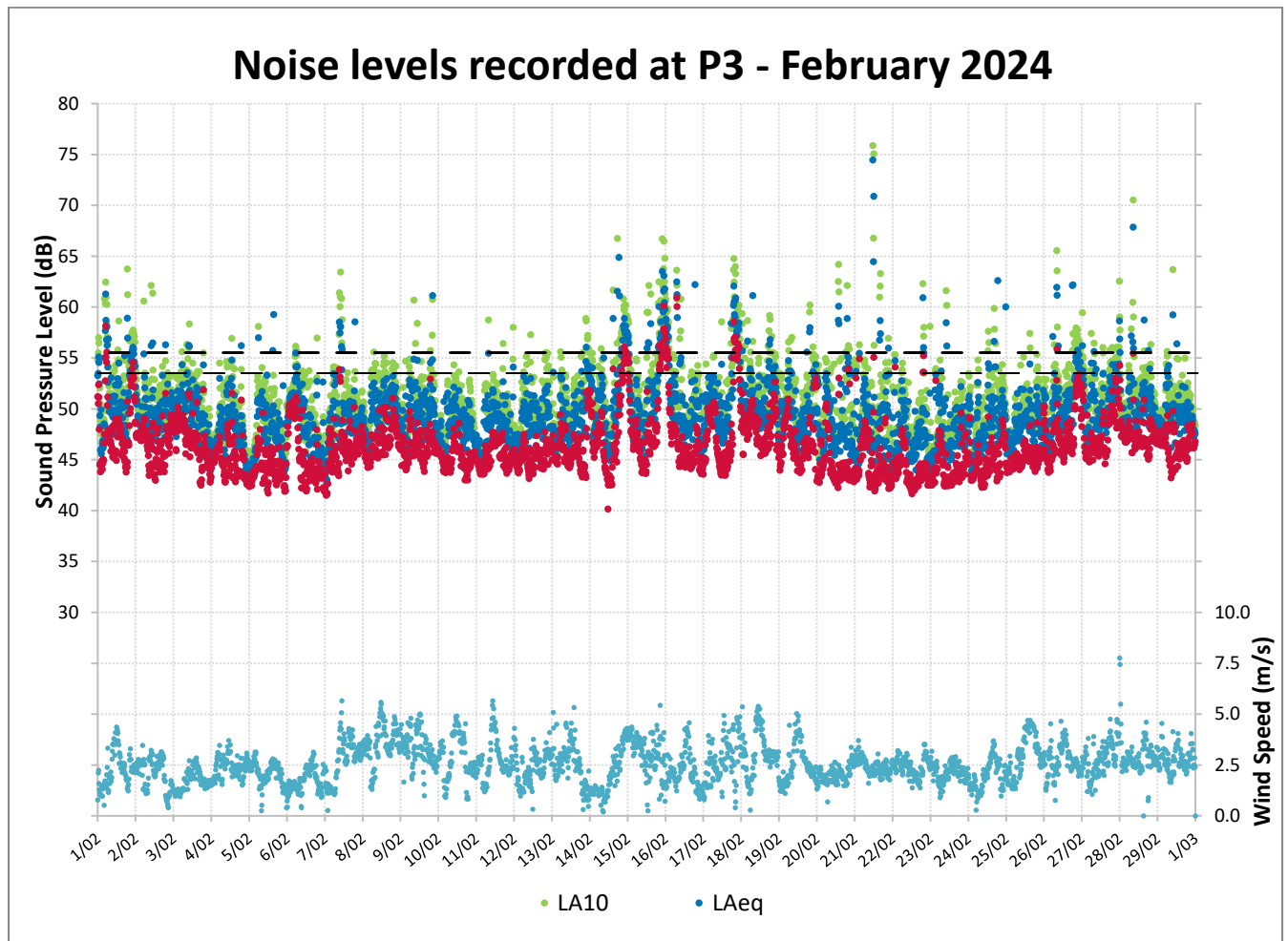
Figure 9: Noise Levels Recorded at P3 for February 2024
