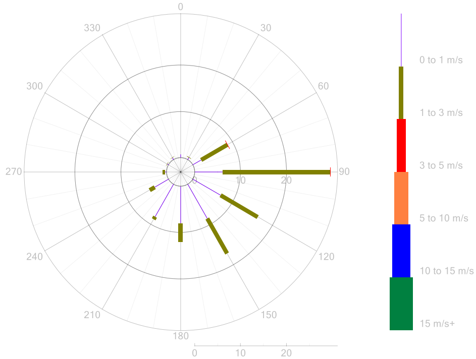
Figure 12: P2 Wind Rose 5-Minute Data for February 2024
