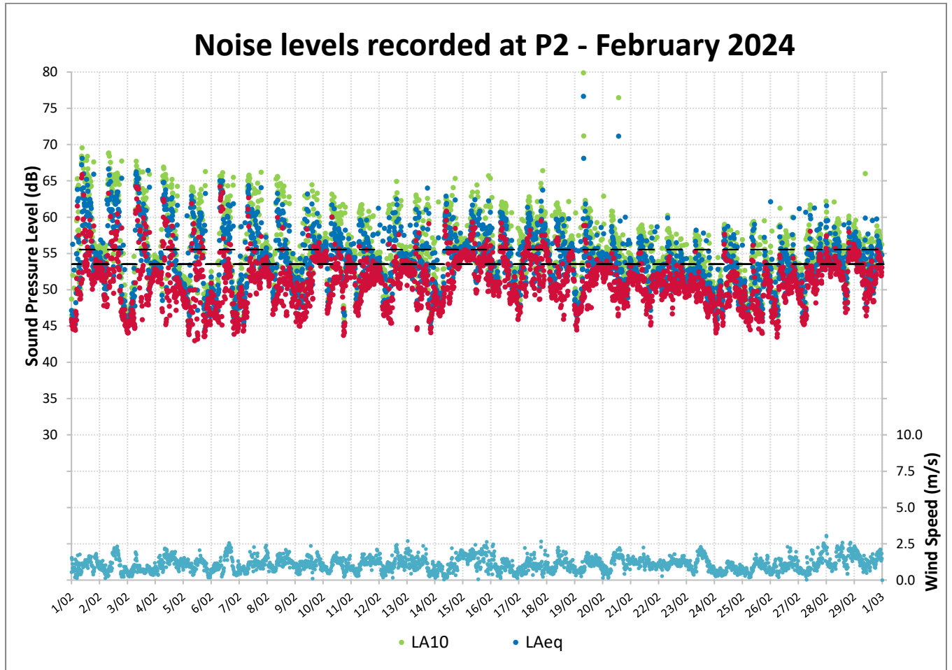
Figure 8: Noise Levels Recorded at P2 for February 2024
