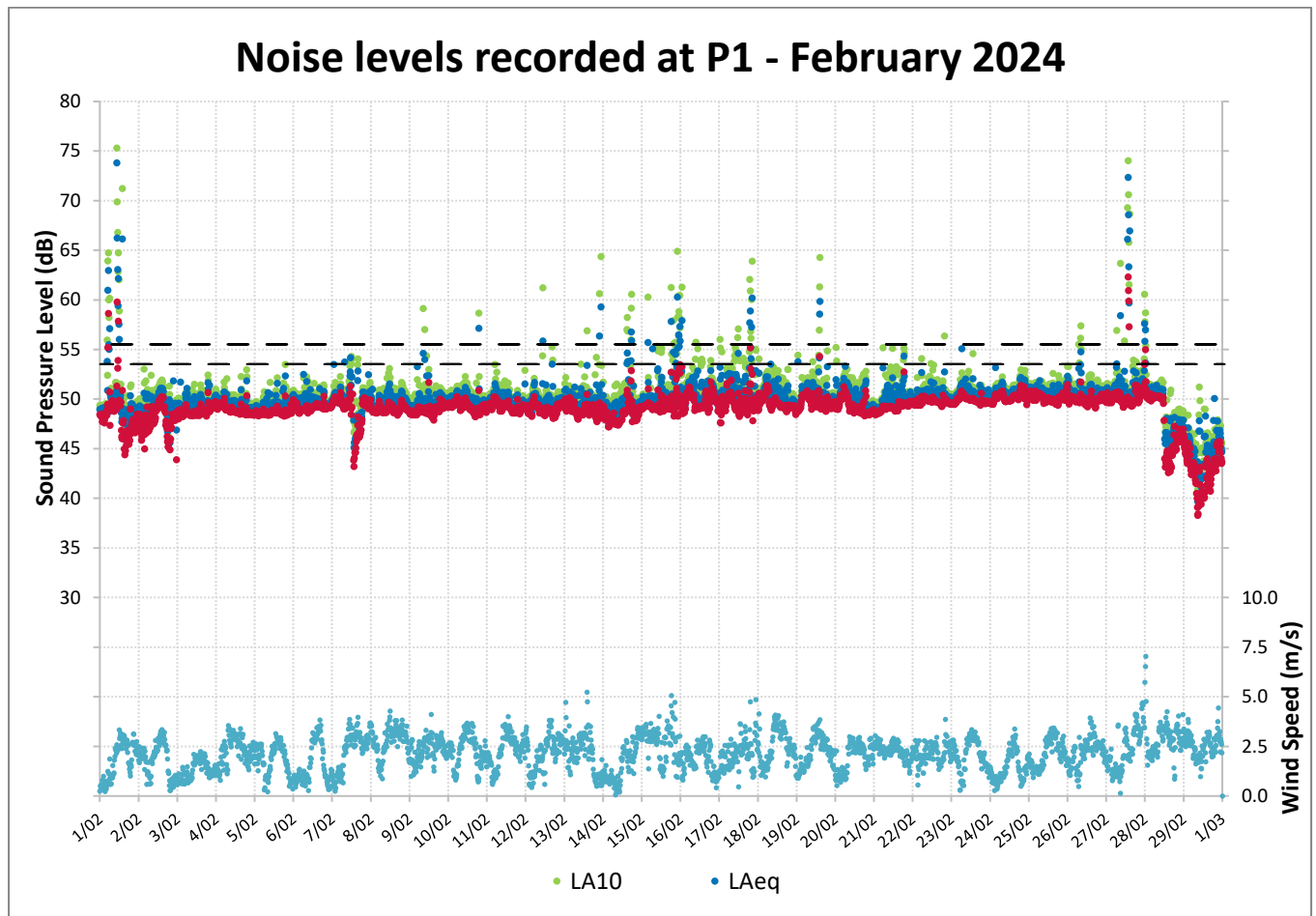
Figure 7: Noise Levels Recorded at P1 for February 2024 8
