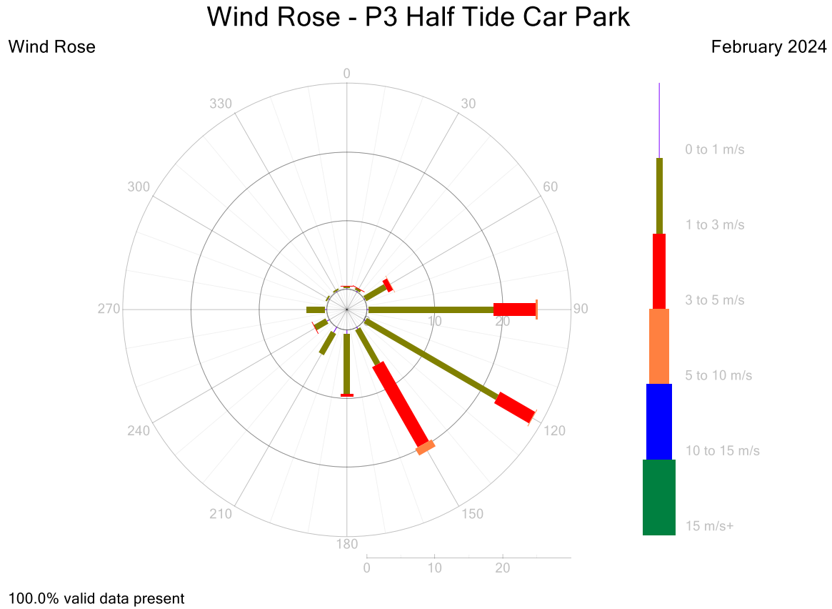
Figure 13: P3 Wind Rose 5-Minute Data for February 2024
