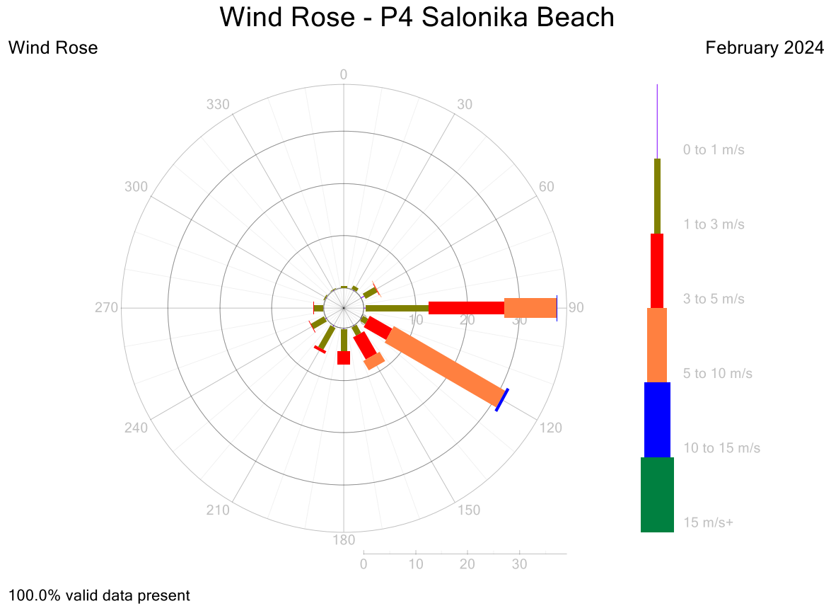
Figure 14: P4 Wind Rose 5-Minute Data for February 2024
