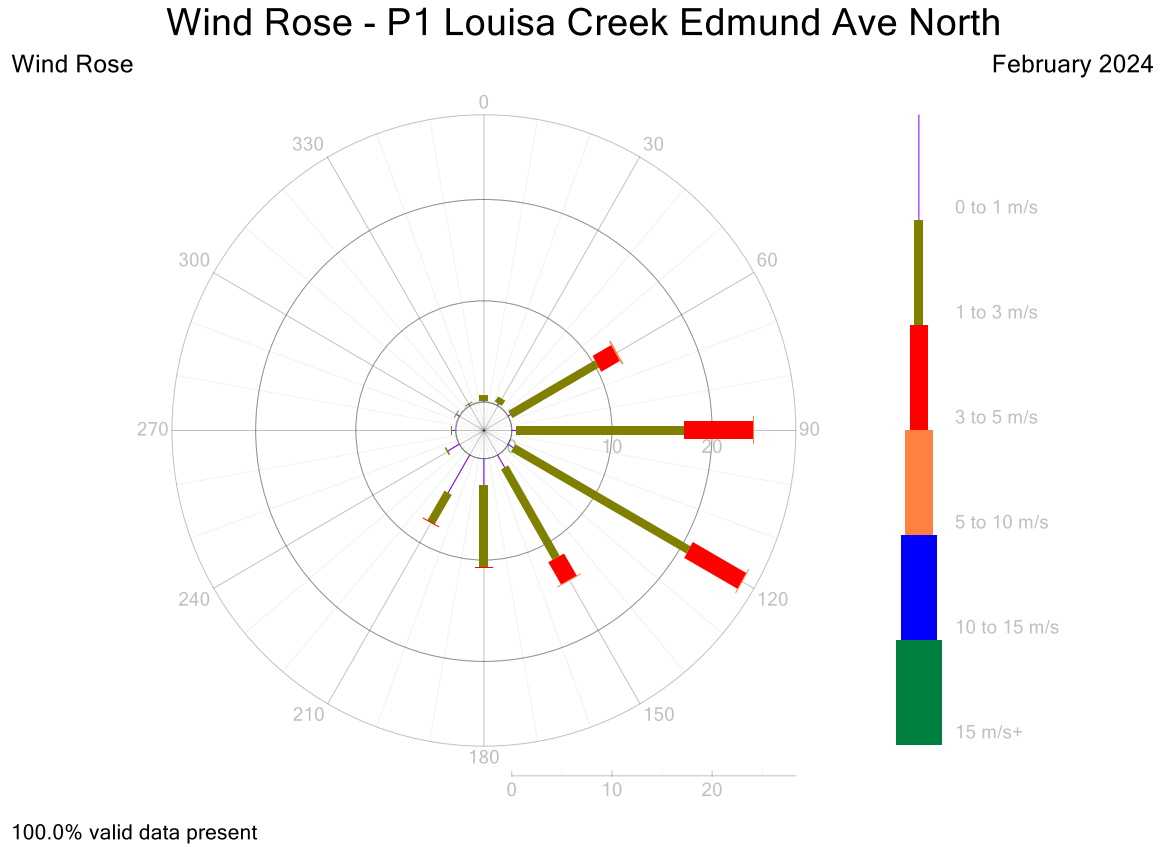
Figure 11: P1 Wind Rose 5-Minute Data for February 2024
