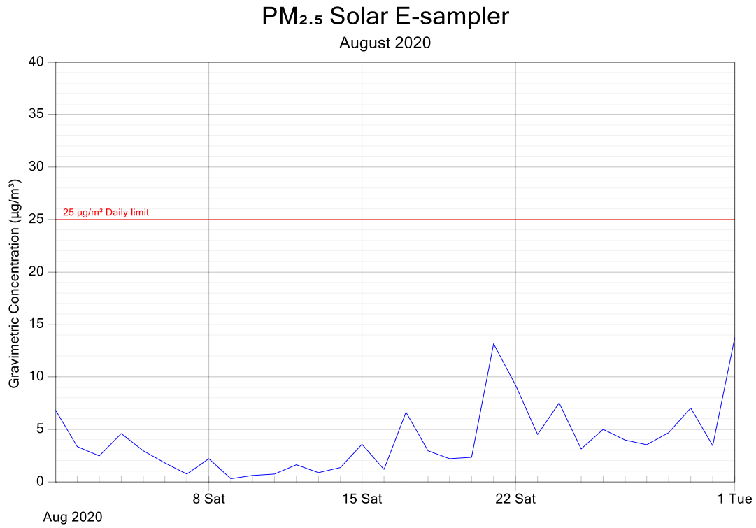
Figure 6: PM 2.5 for McEwens Beach Station 24-hour Averages – August 2020
