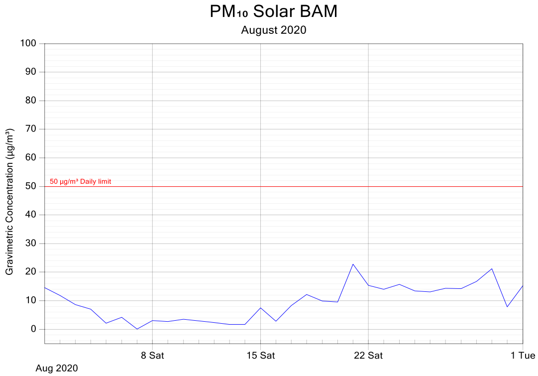
Figure 4: PM 10 for McEwens Beach station 24-hour Averages – August 2020
