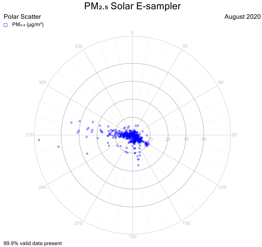
Figure 5: PM 2.5 Polar Scatter Plot (1-Hour Average) for McEwens Beach Station – August 2020
