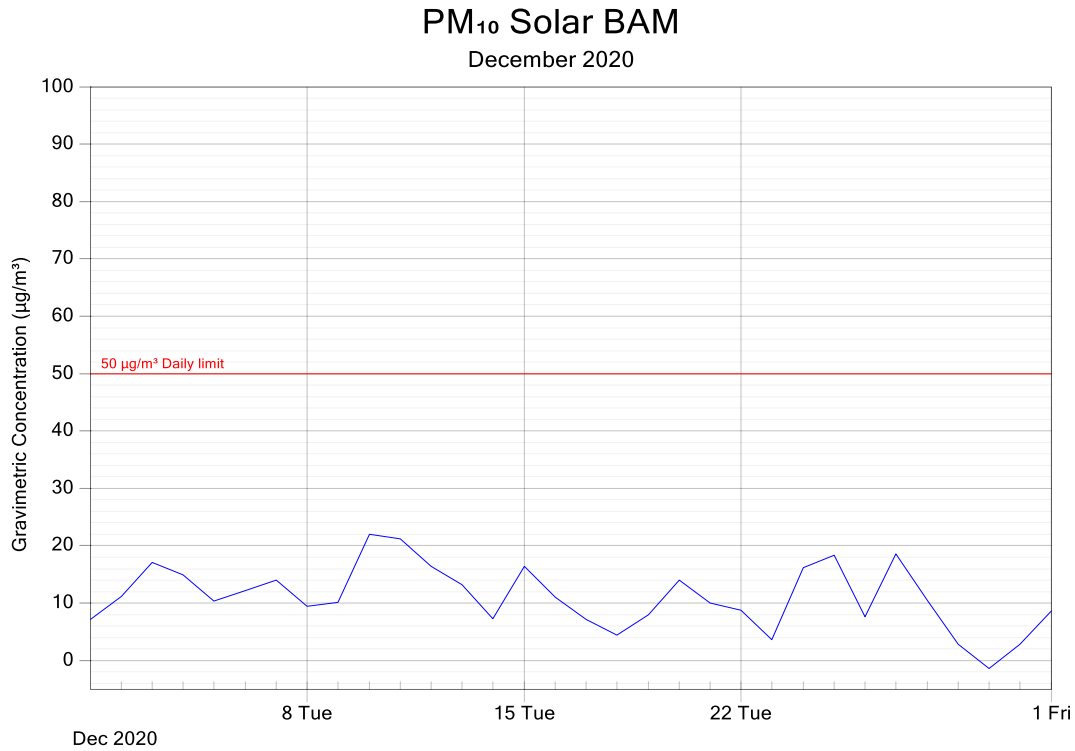
Figure 2: PM 10 for McEwens Beach station 24-hour Averages – December 2020
