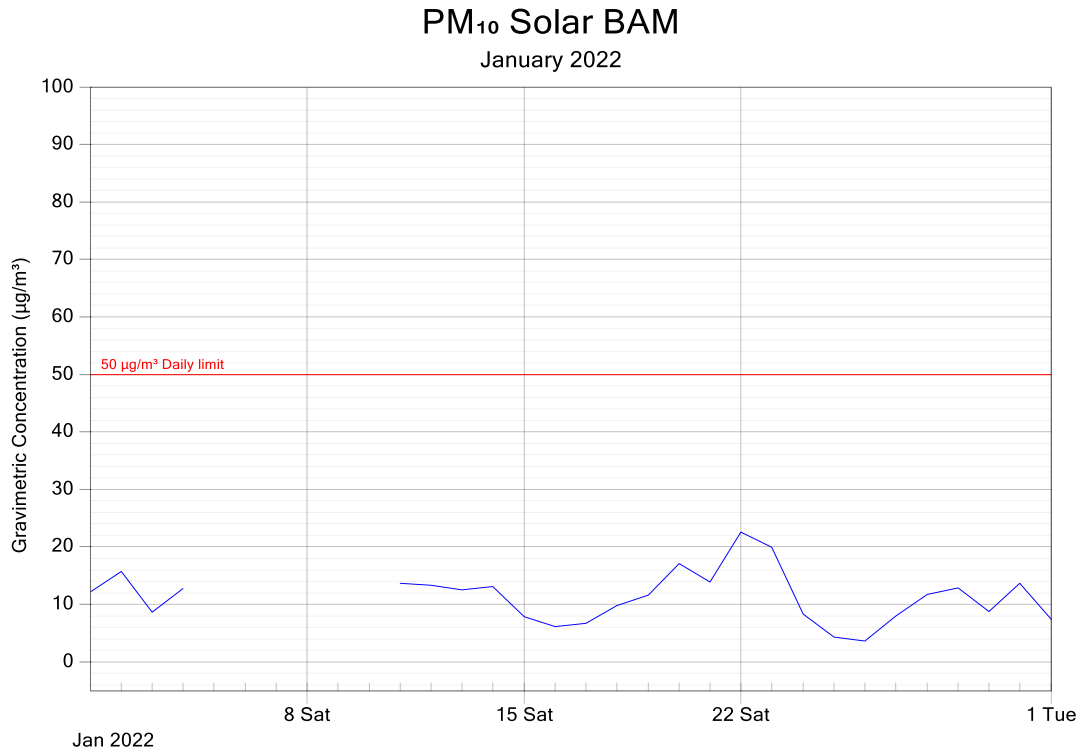
Figure 2: PM 10 for McEwens Beach station 24-hour Averages – January 2022
