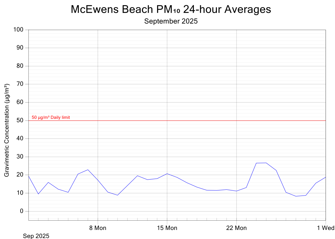
Figure 5: McEwens Beach Station PM 10 24-hour Averages
