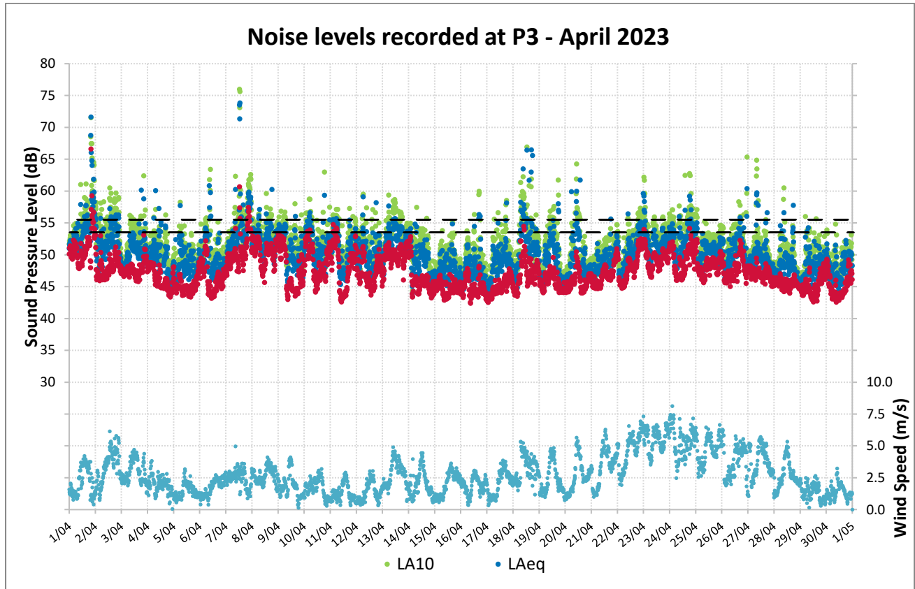
Figure 9: Noise Levels Recorded at P3 for April 2023
