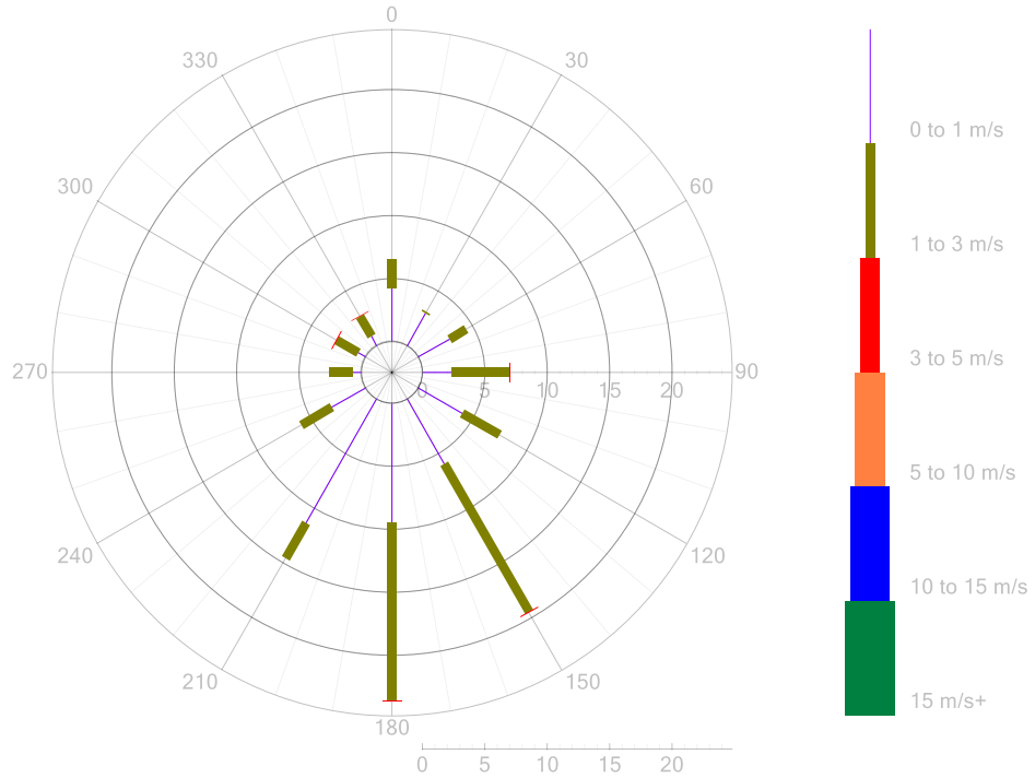
Figure 12: P2 Wind Rose 5-Minute Data for April 2023
