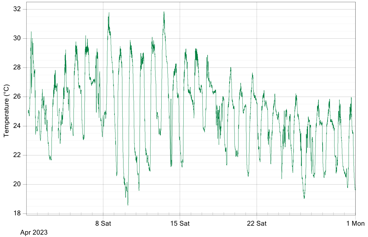
Figure 15: Port of Hay Point AT 5-Minute Averages Data for April 2023
