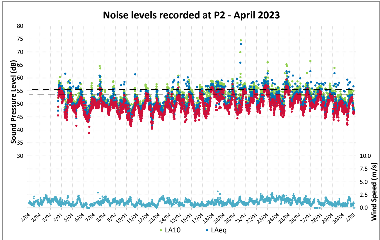
Figure 8: Noise Levels Recorded at P2 for April 2023
