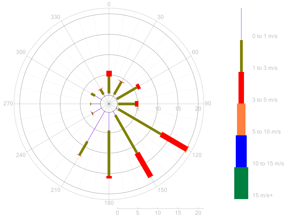
Figure 11: P1 Wind Rose 5-Minute Data for April 2023
