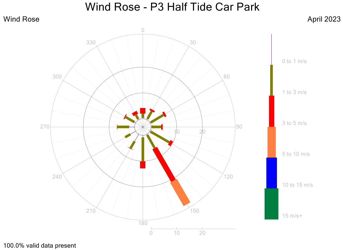
Figure 13: P3 Wind Rose 5-Minute Data for April 2023
