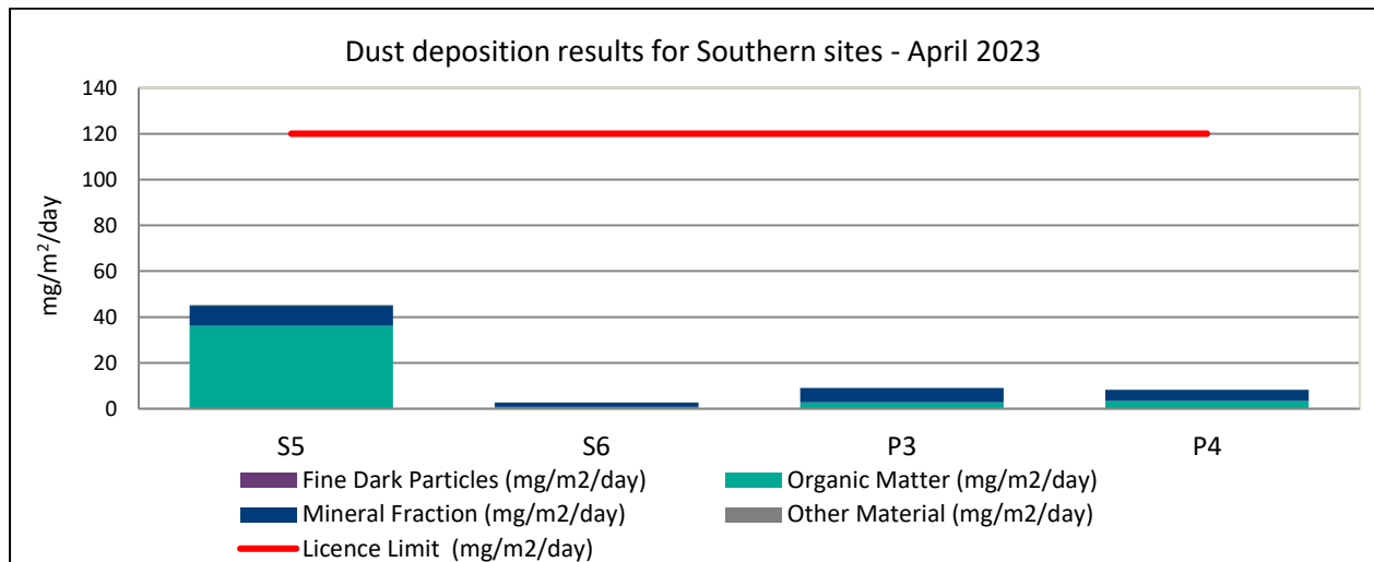
Figure 6: Dust Deposition Results for Southern Sites, April 2023
