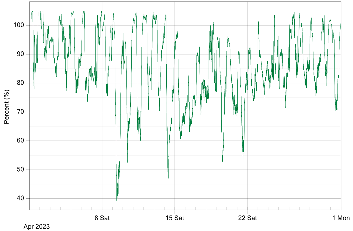
Figure 16: Port of Hay Point RH 5-Minute Averages Data for April 2023
