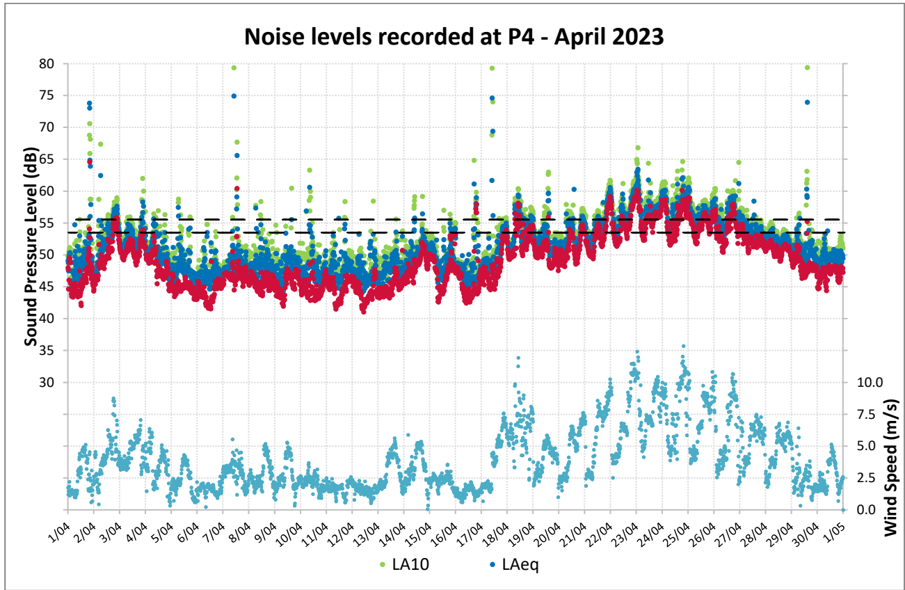
Figure 10: Noise Levels Recorded at P4 for April 2023
