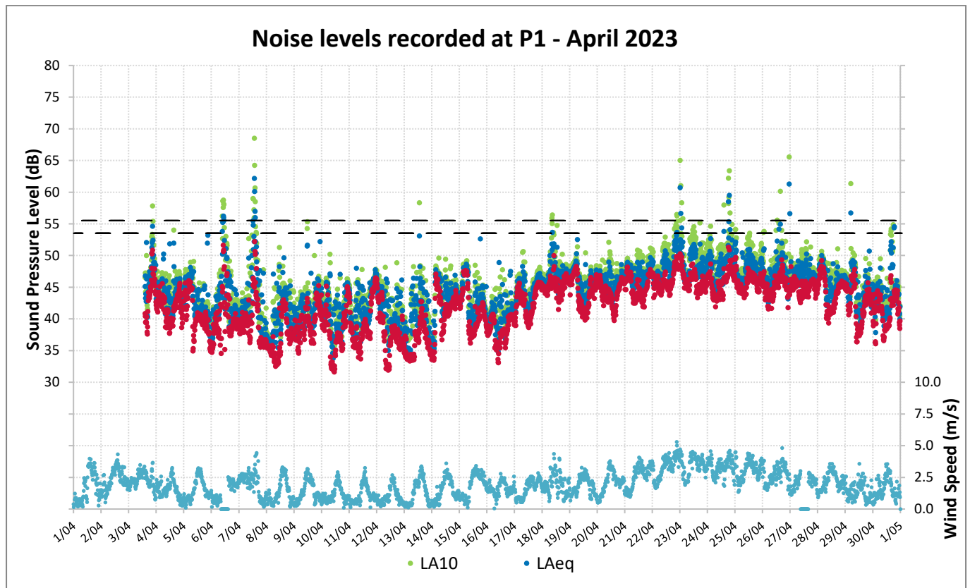
Figure 7: Noise Levels Recorded at P1 for April 2023
