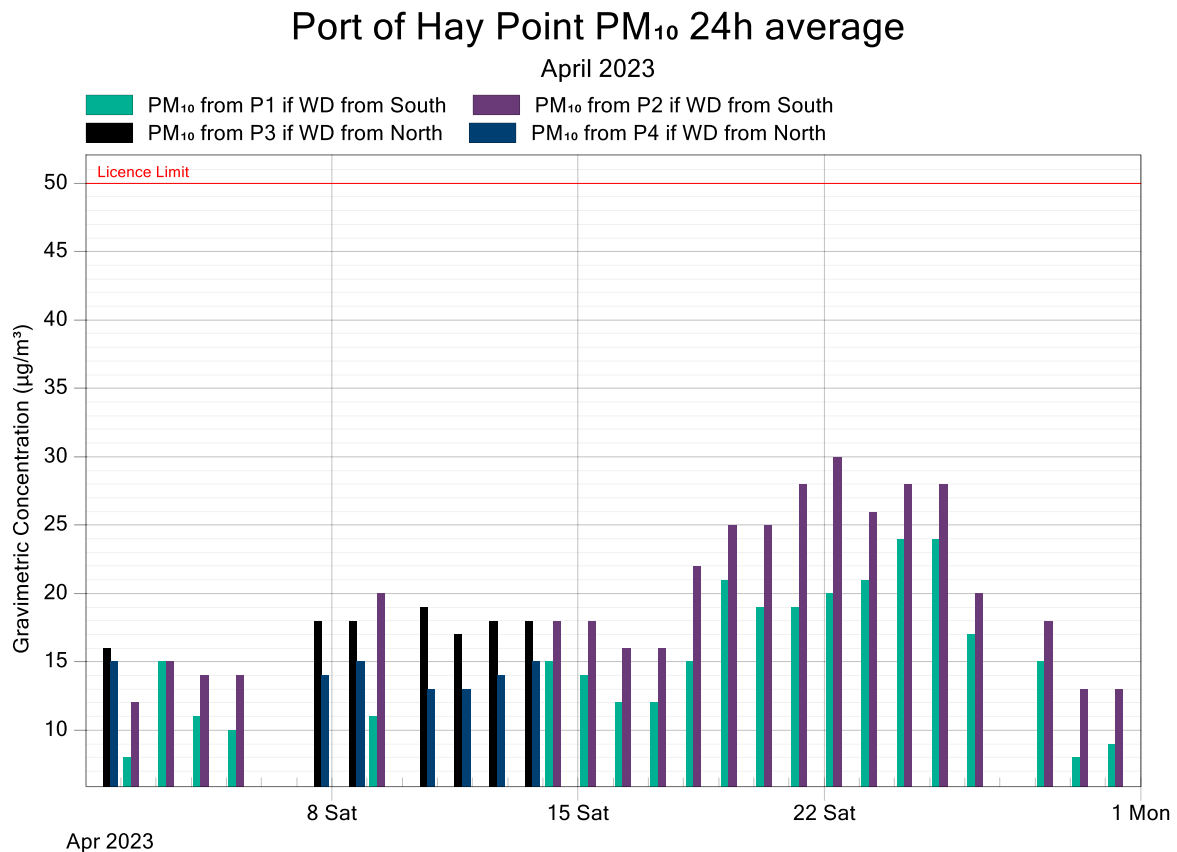
Figure 4: Port of Hay Point PM 10 24-Hour Average Data Compared to the Licence Limit for April 2023
