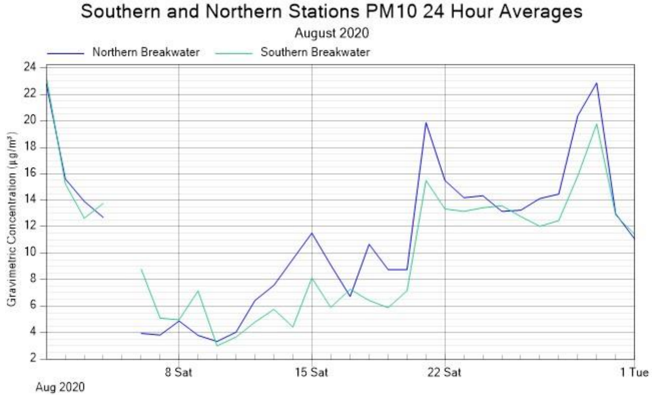
Figure 6: Southern and Northern Stations PM 10 24 Hour Averages Comparison August 2020
