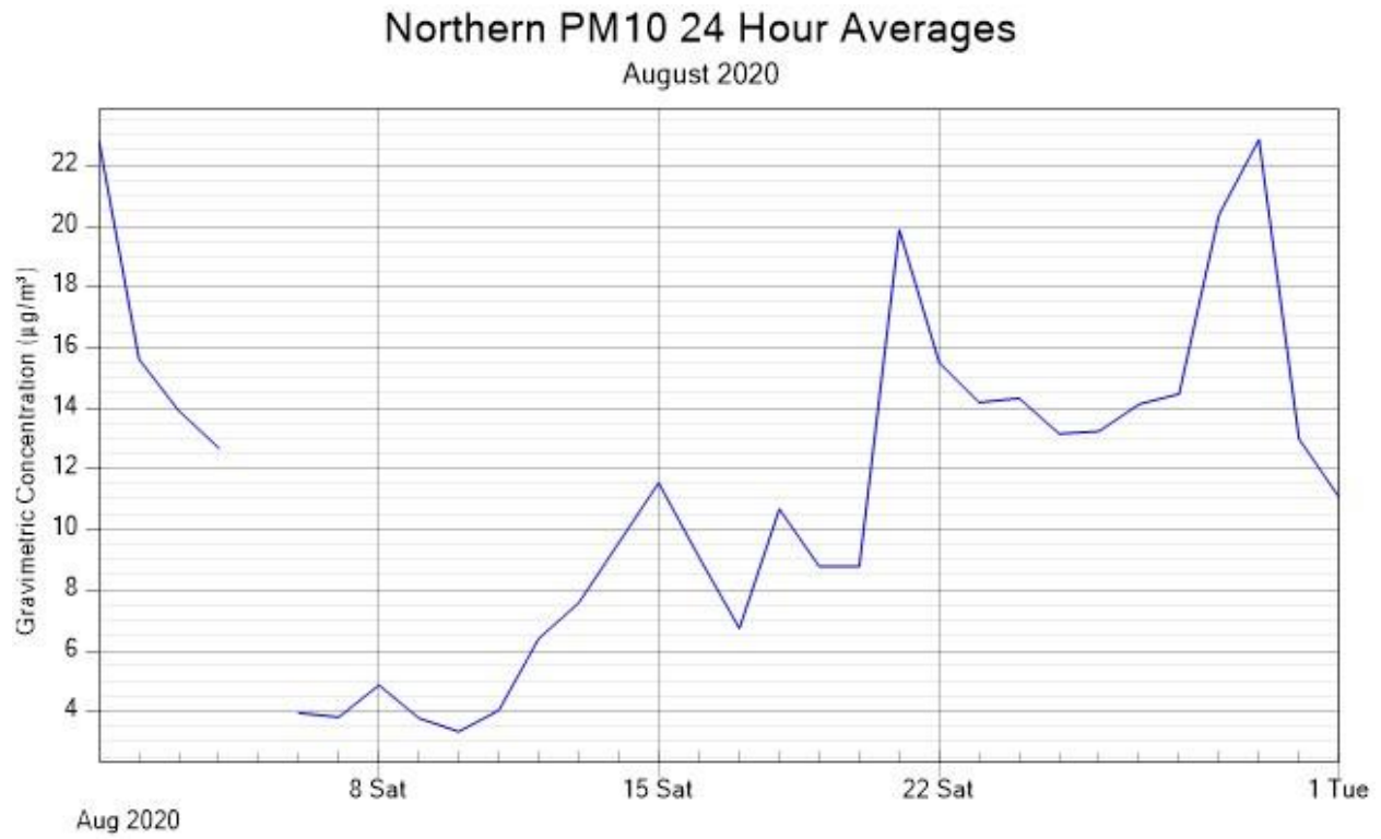
Figure 5: Northern station PM 10 24 Hour Averages August 2020
