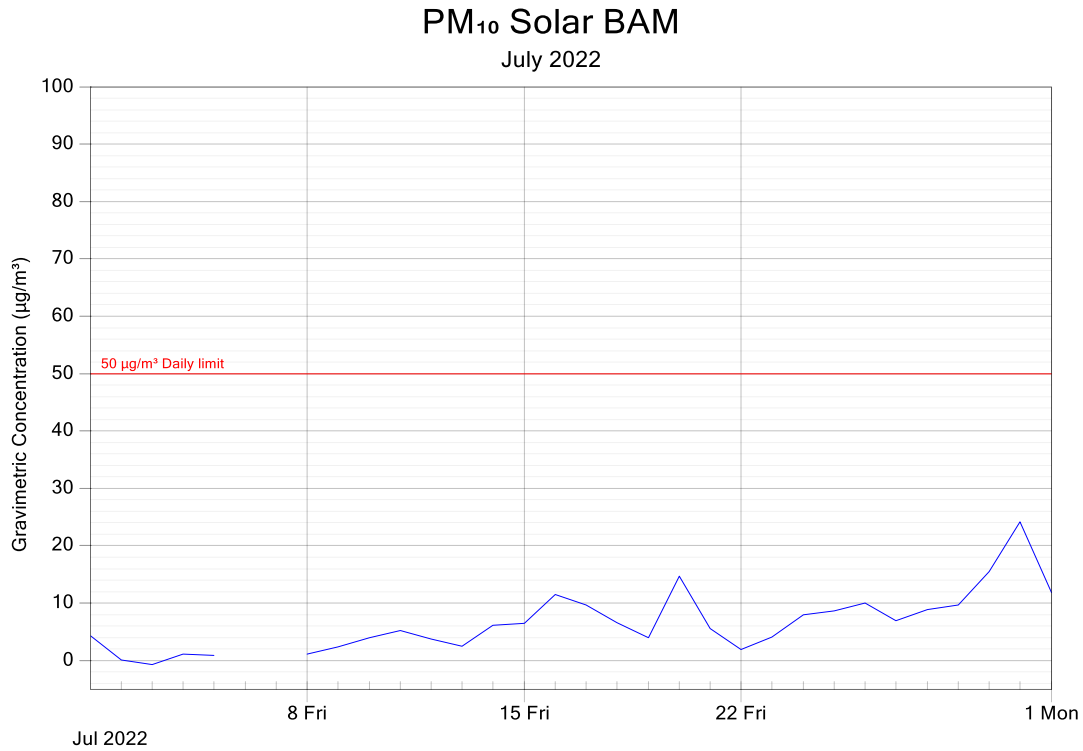
Figure 2: PM 10 for McEwens Beach station 24-hour Averages – July 2022
