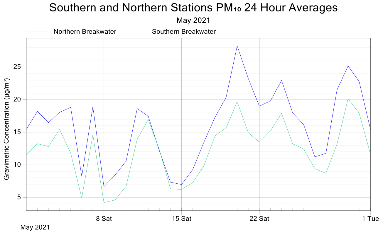
Figure 6: Southern and Northern Stations PM 10 24 Hour Averages Comparison May 2021
