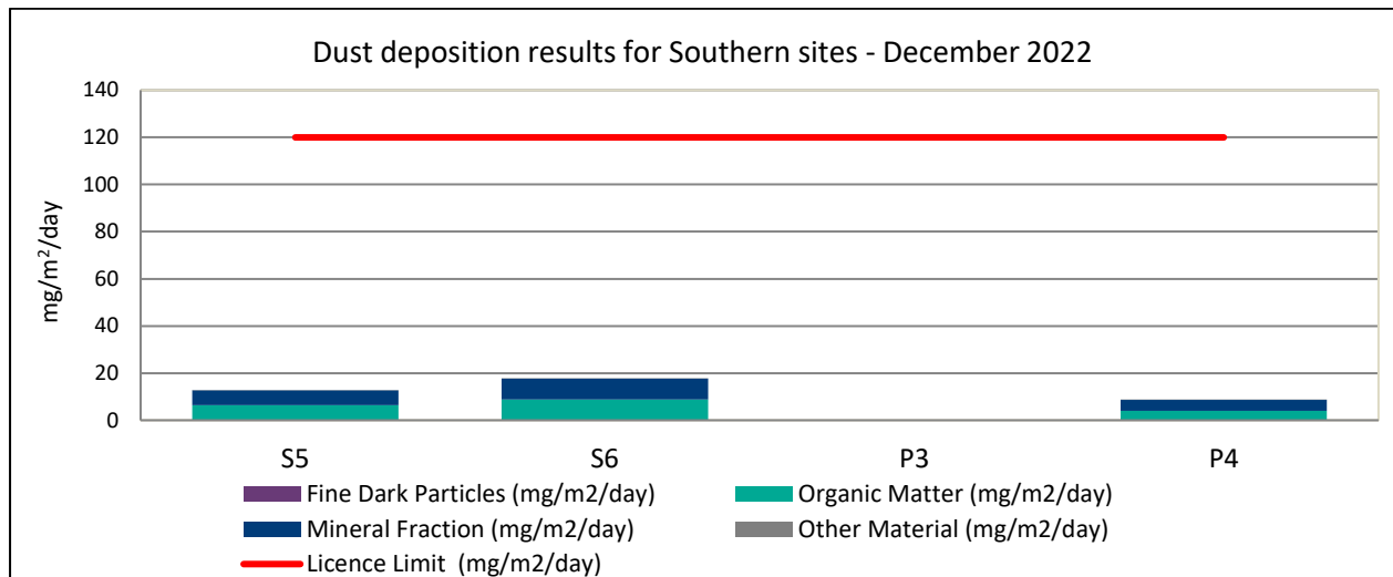
Figure 6: Dust Deposition Results for Southern Sites, December 2022 7
