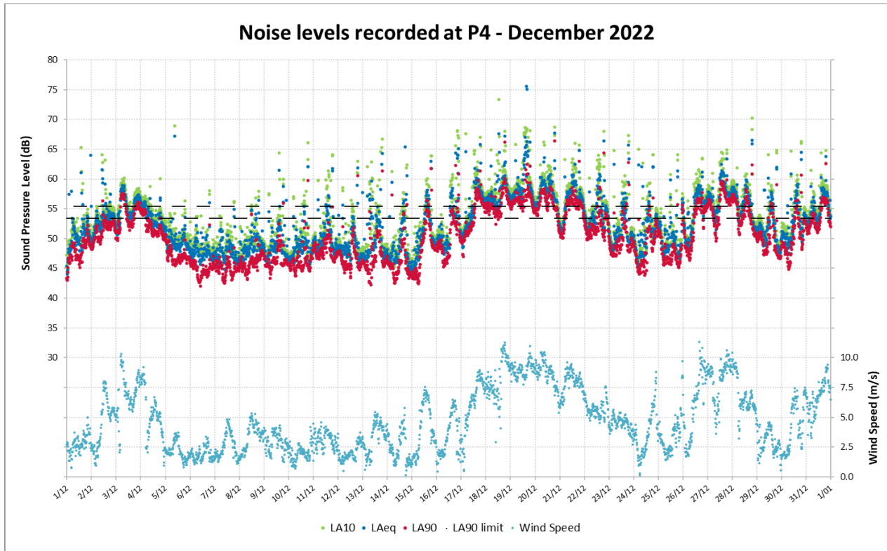
Figure 10: Noise Levels Recorded at P4 for December 2022
