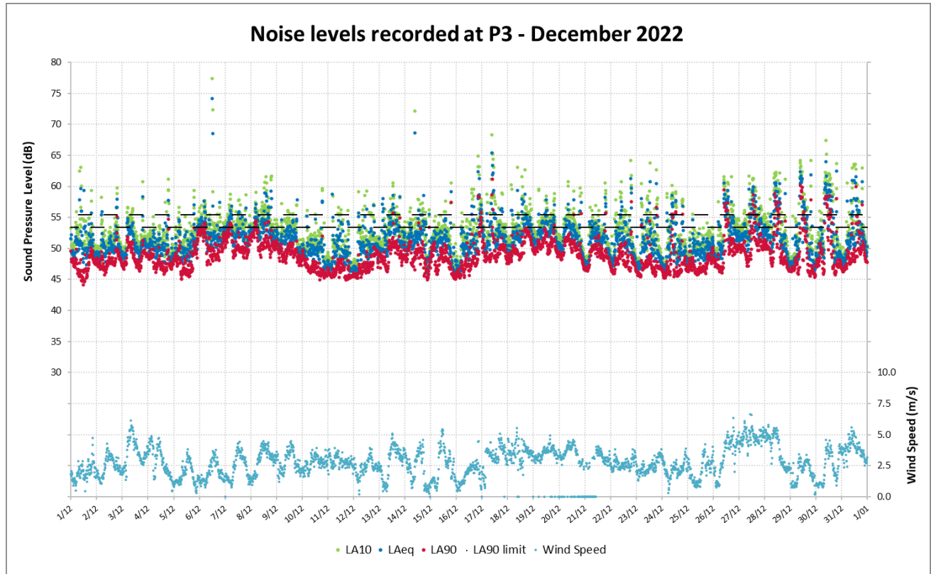
Figure 9: Noise Levels Recorded at P3 for December 2022
