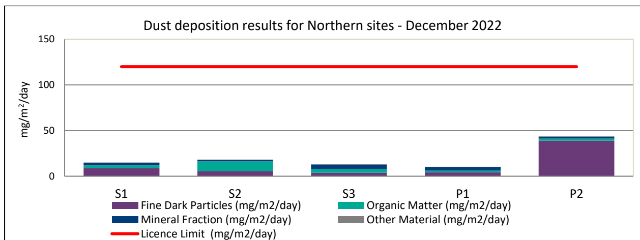
Figure 5: Dust Deposition Results for Northern Sites, December 2022
