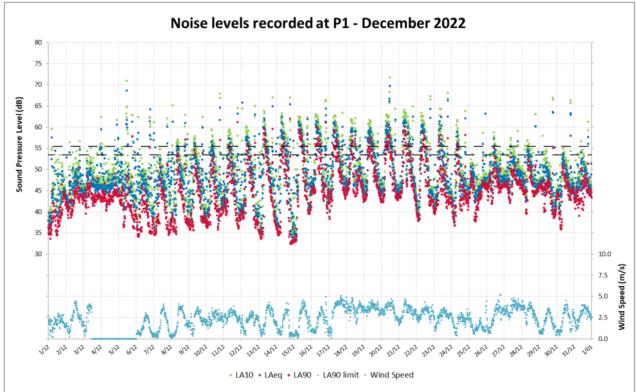
Figure 7: Noise Levels Recorded at P1 for December 2022
