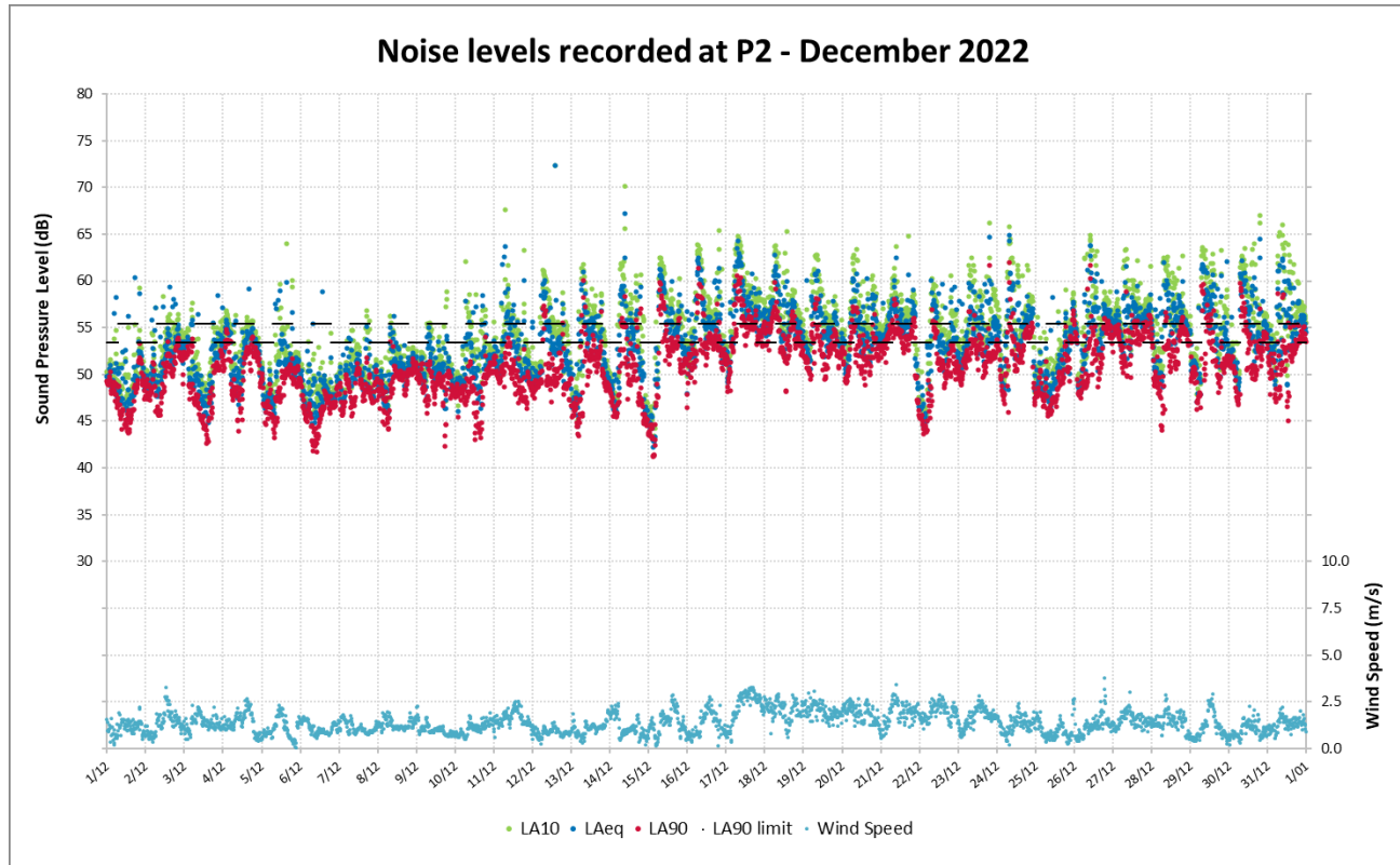
Figure 8: Noise Levels Recorded at P2 for December 2022
