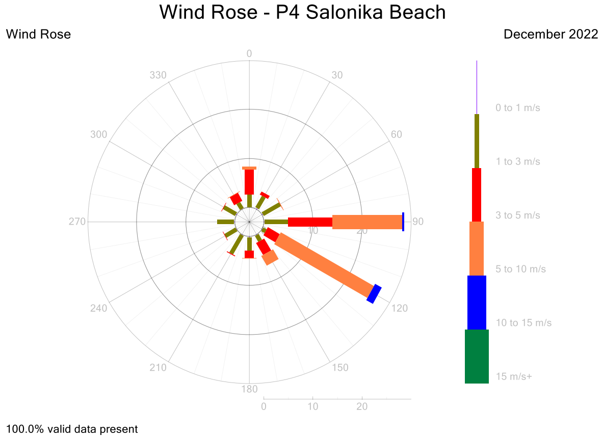
Figure 14: P4 Wind Rose 5-Minute Data for December 2022
