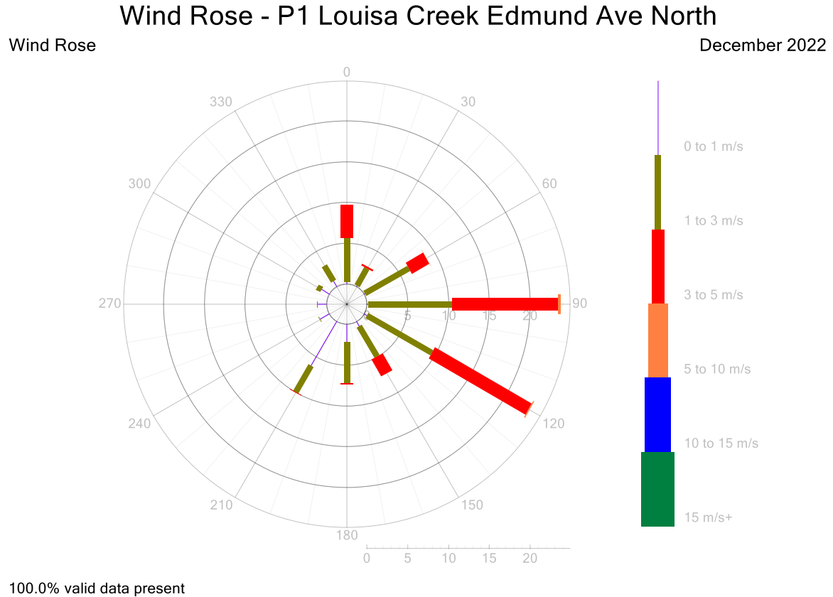
Figure 11: P1 Wind Rose 5-Minute Data for December 2022
