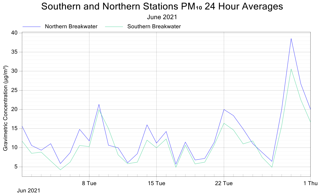
Figure 6: Southern and Northern Stations PM 10 24 Hour Averages Comparison June 2021
