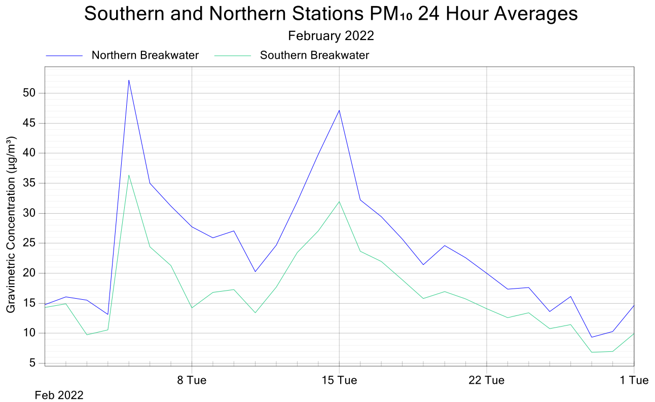
Figure 6: Southern and Northern Stations PM 10 24 Hour Averages Comparison February 2022
