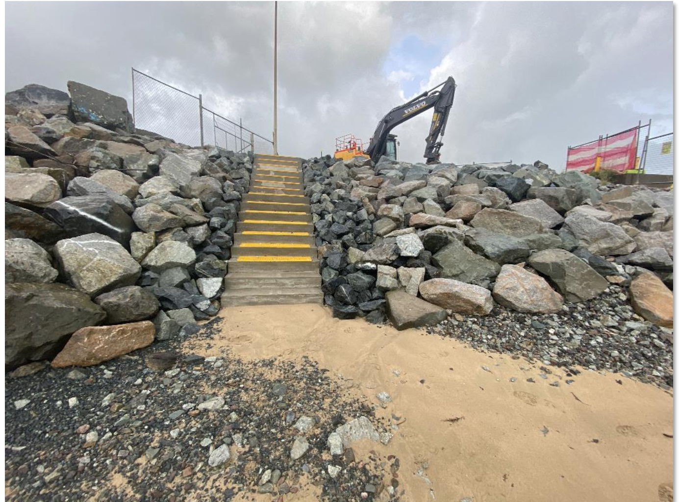
Half Tide steps construction works.
