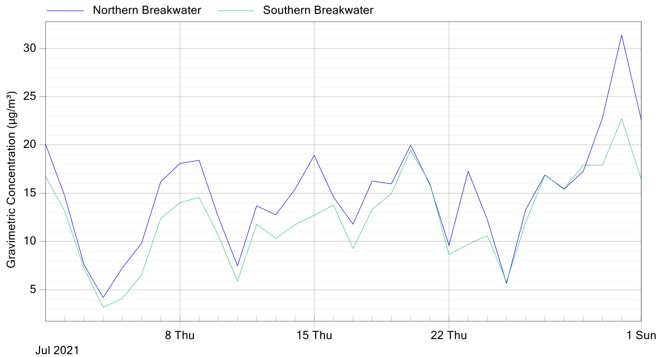
Figure 6: Southern and Northern Stations PM 10 24 Hour Averages Comparison July 2021
