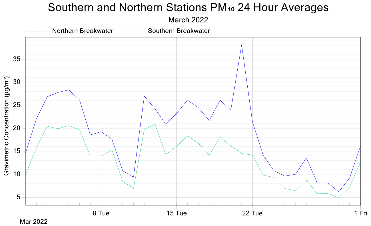
Figure 6: Southern and Northern Stations PM 10 24 Hour Averages Comparison March 2022
