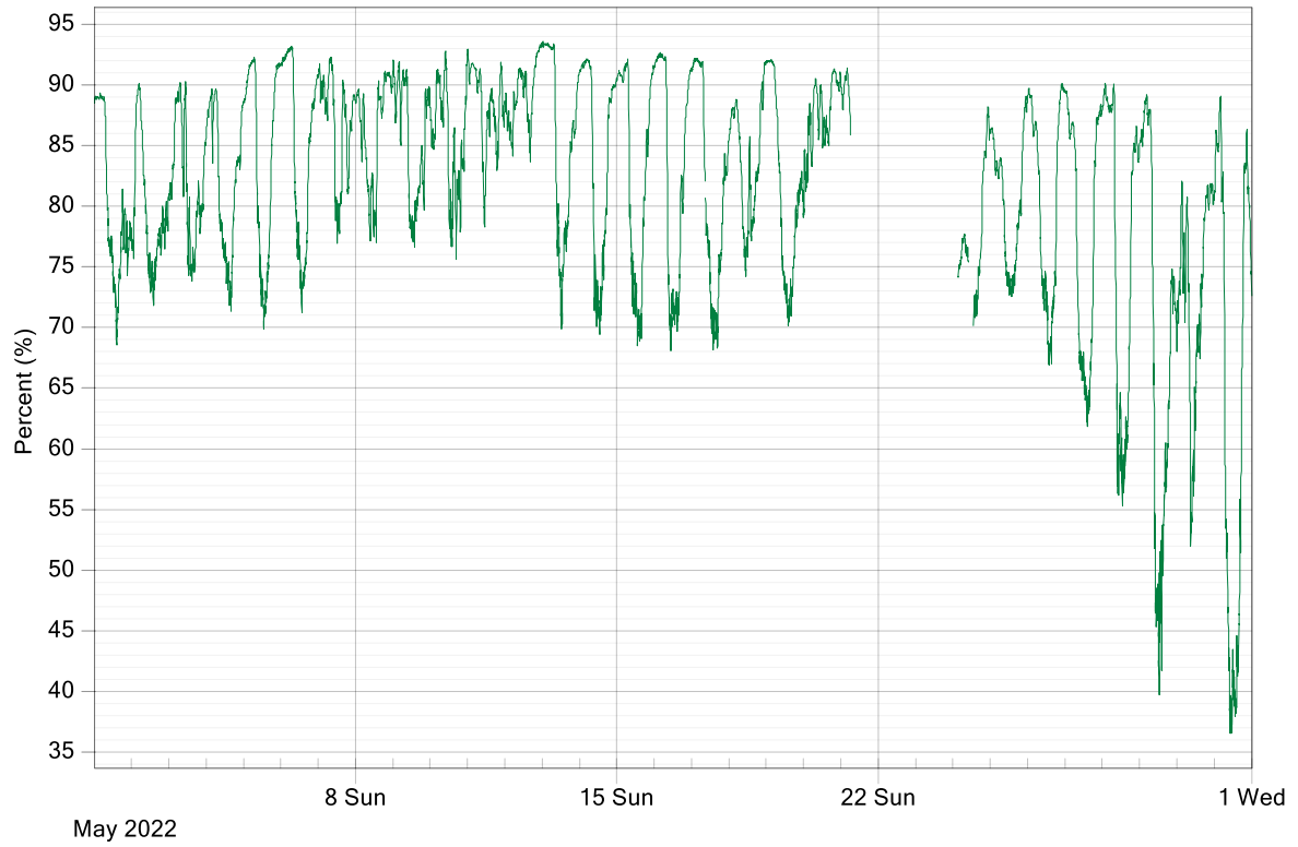
Figure 16: Port of Hay Point RH 5-Minute Averages Data for May 2022
