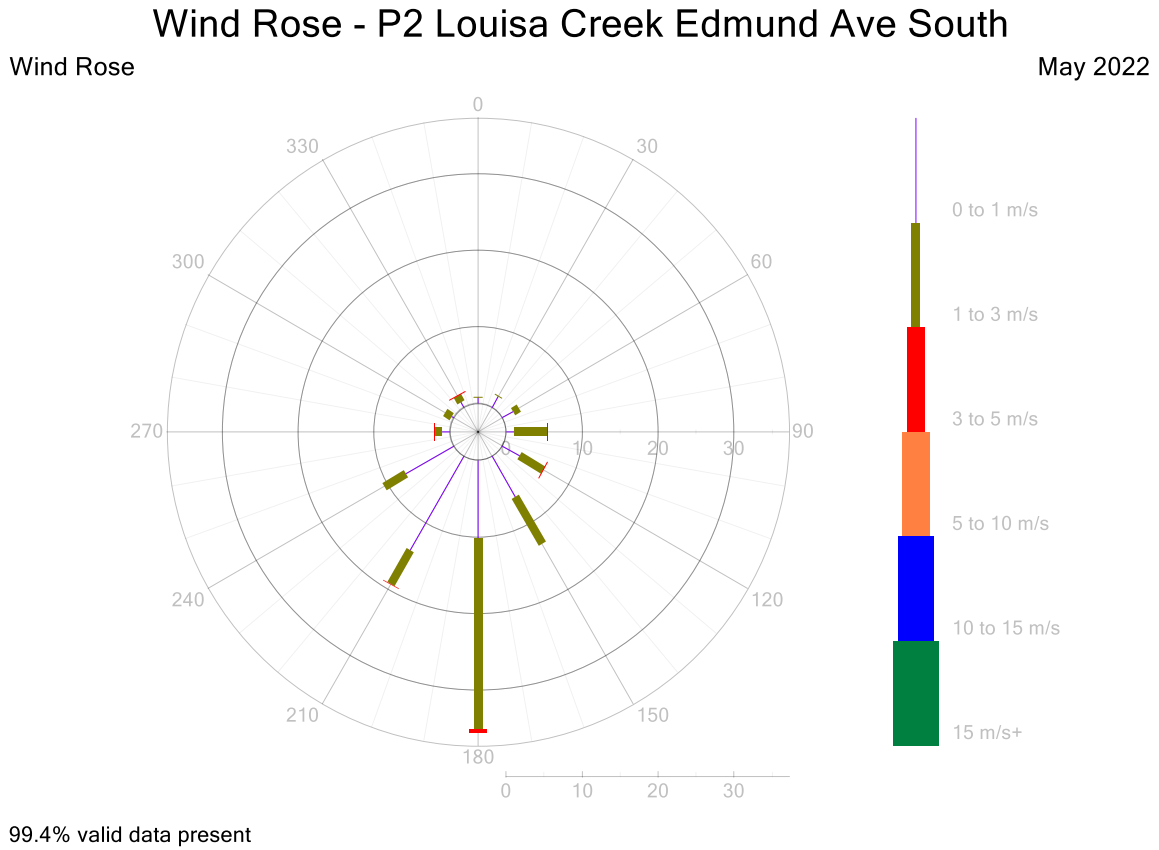
Figure 12: P2 Wind Rose 5-Minute Data for May 2022
