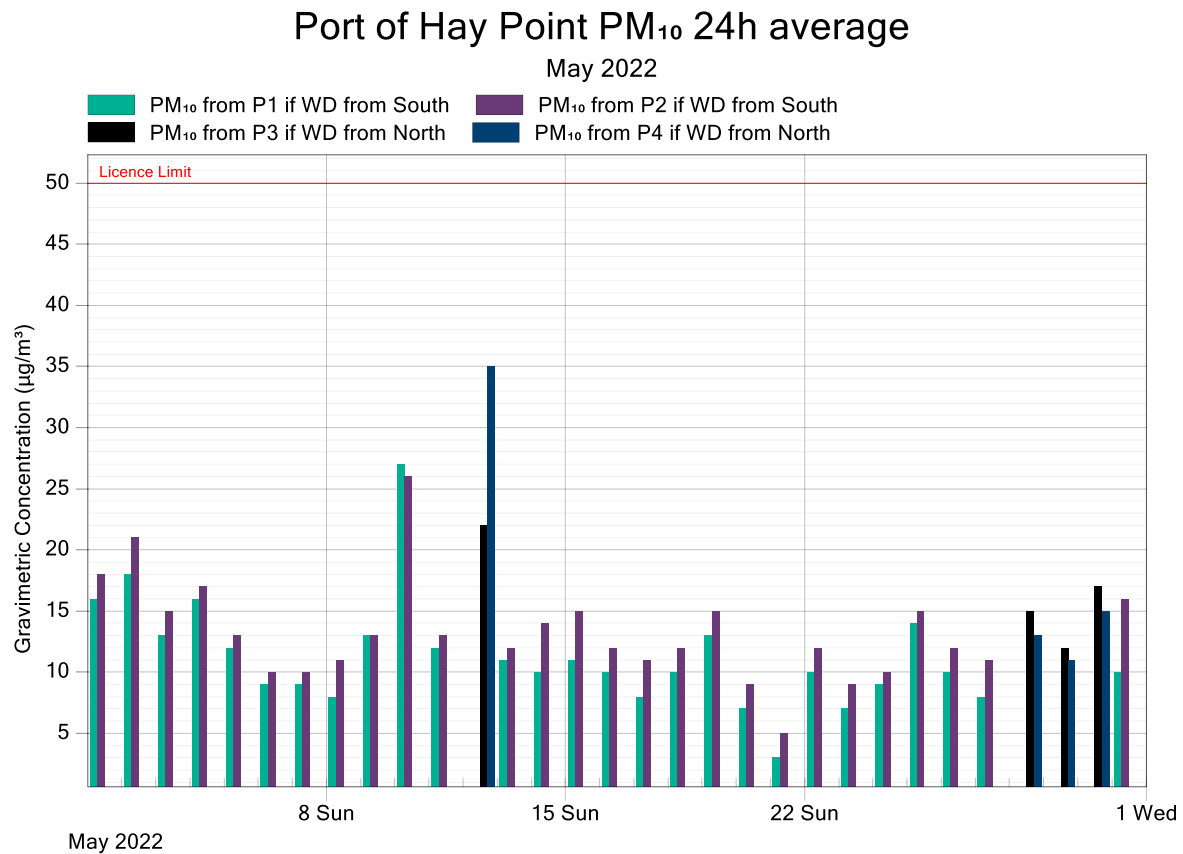
Figure 4: Port of Hay Point PM 10 24-Hour Average Data Compared to the Licence Limit for May 2022
