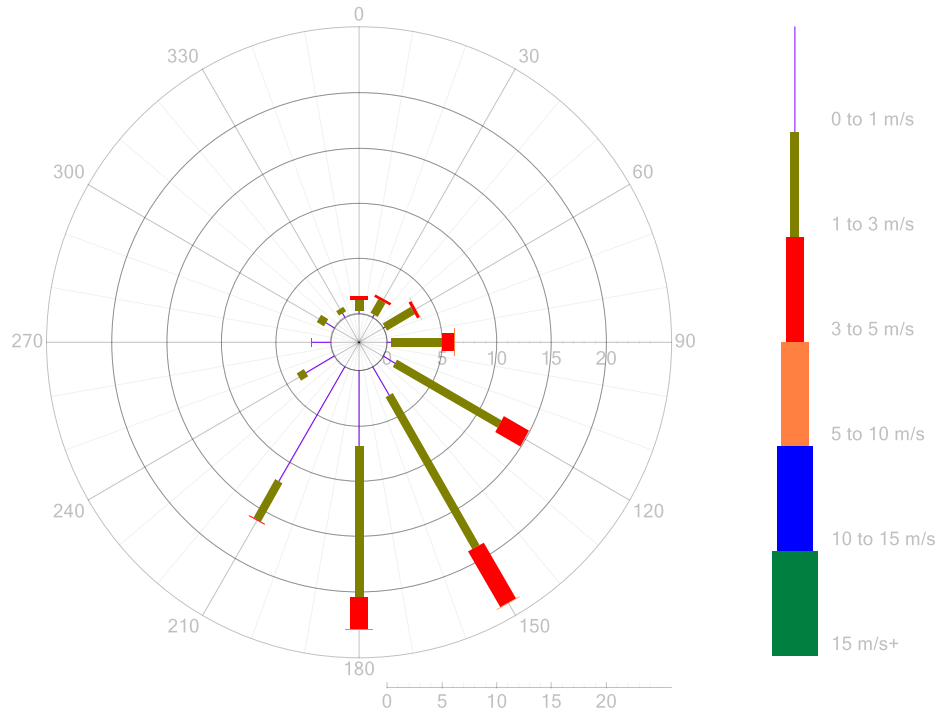
Figure 11: P1 Wind Rose 5-Minute Data for May 2022
