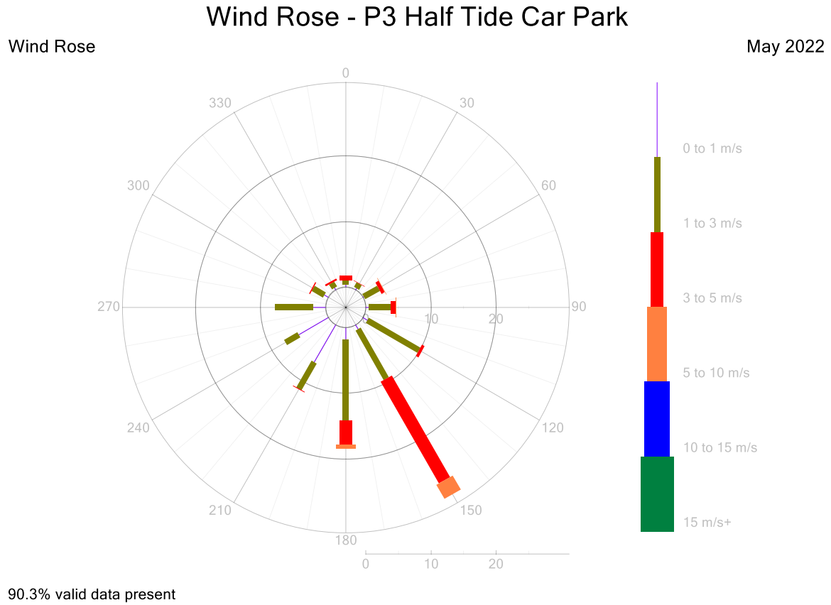
Figure 13: P3 Wind Rose 5-Minute Data for May 2022
