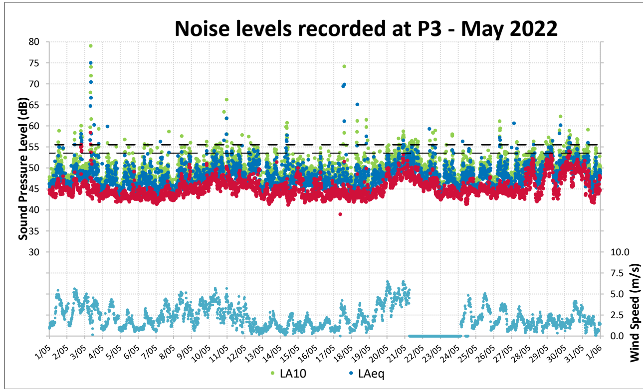
Figure 9: Noise Levels Recorded at P3 for May 2022
