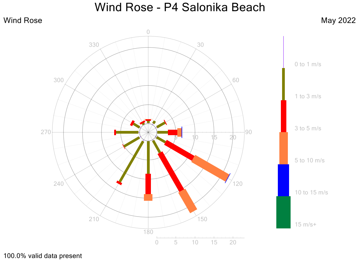
Figure 14: P4 Wind Rose 5-Minute Data for May 2022
