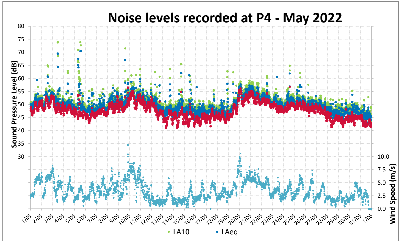
Figure 10: Noise Levels Recorded at P4 for May 2022
