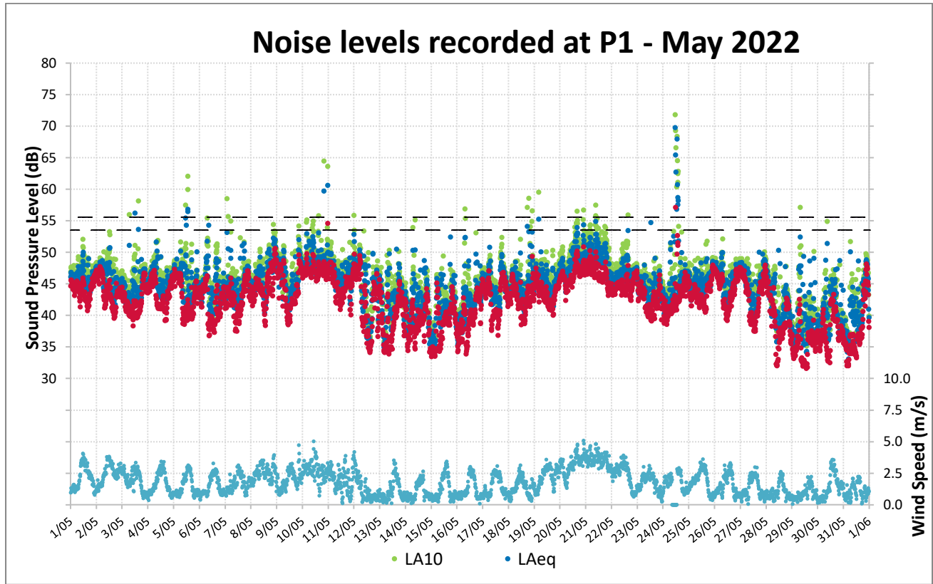
Figure 7: Noise Levels Recorded at P1 for May 2022
