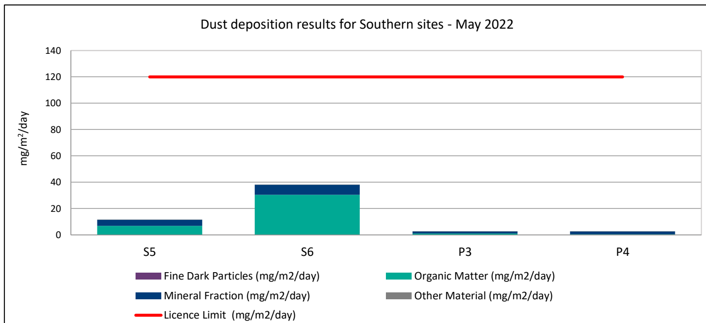
Figure 6: Dust Deposition Results for Southern Sites, May 2022
