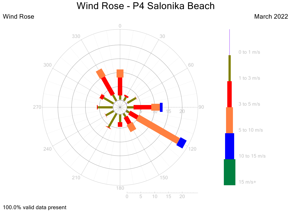
Figure 14: P4 Wind Rose 5-Minute Data for March 2022
