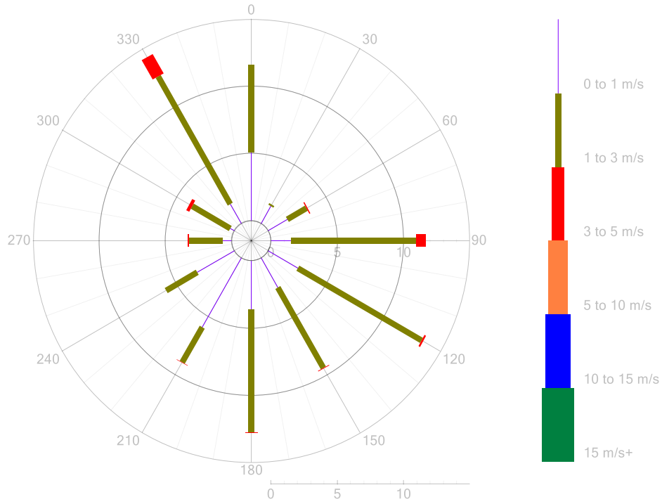
Figure 12: P2 Wind Rose 5-Minute Data for March 2022
