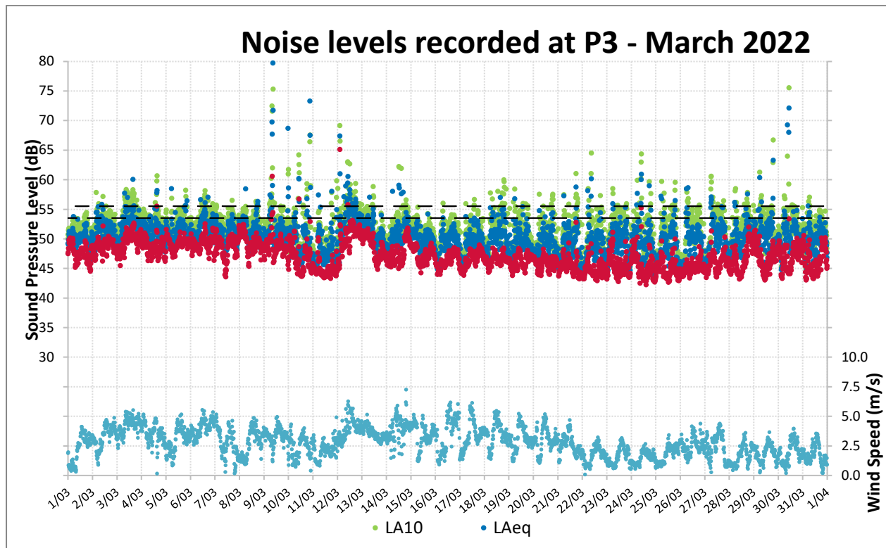
Figure 9: Noise Levels Recorded at P3 for March 2022
