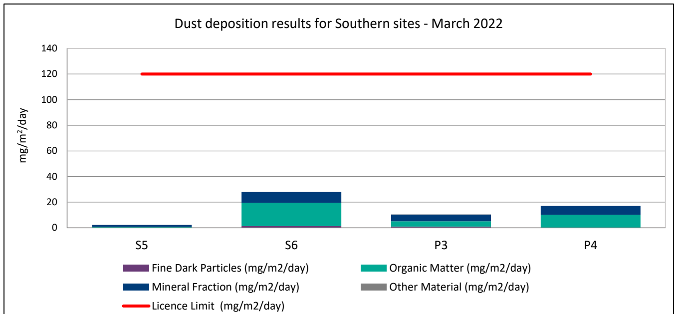
Figure 6: Dust Deposition Results for Southern Sites, March 2022
