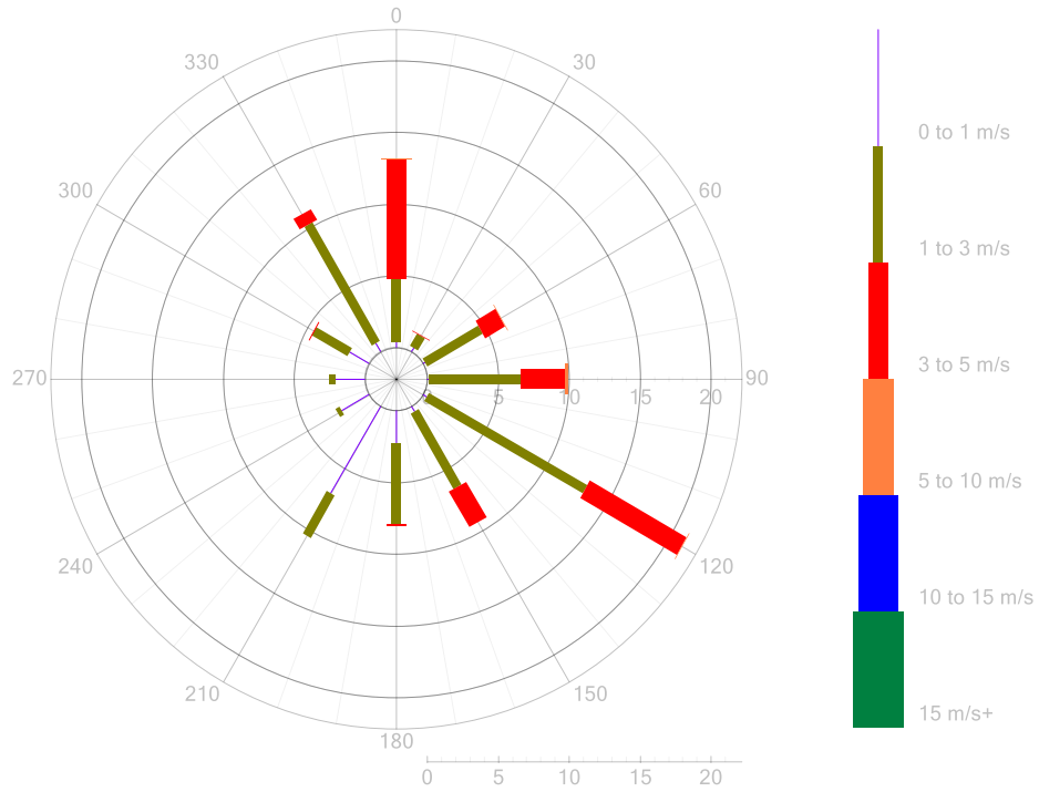
Figure 11: P1 Wind Rose 5-Minute Data for March 2022
