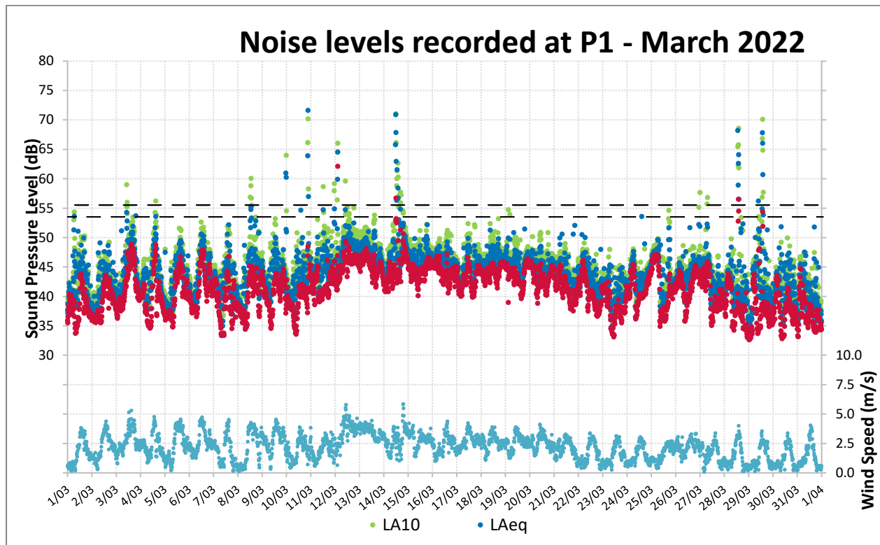
Figure 7: Noise Levels Recorded at P1 for March 2022
