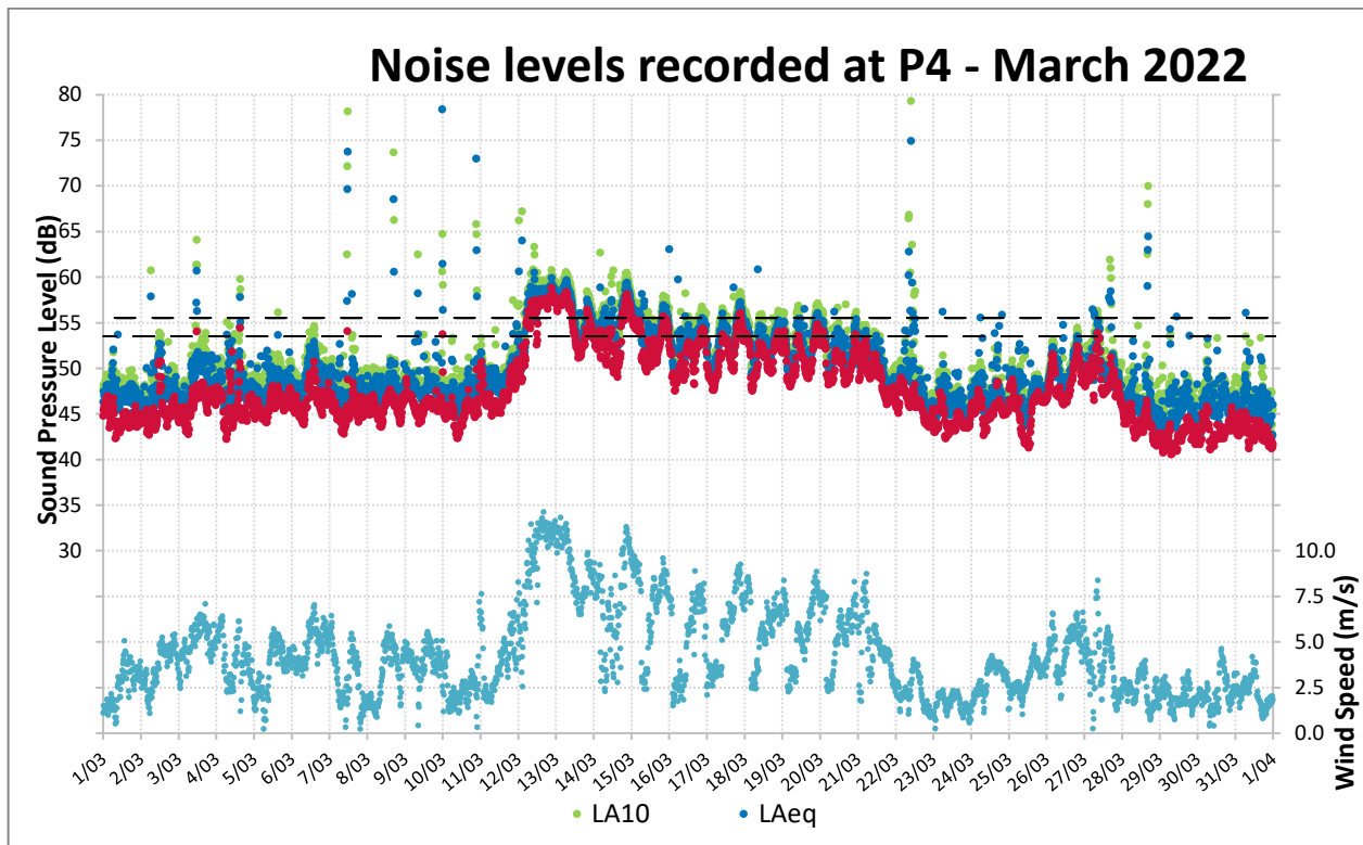
Figure 10: Noise Levels Recorded at P4 for March 2022
