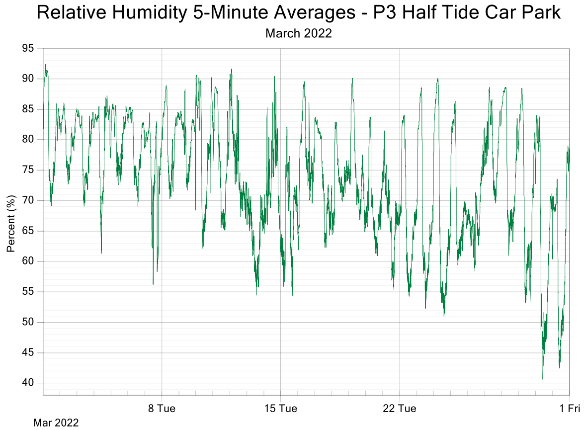
Figure 16: Port of Hay Point RH 5-Minute Averages Data for March 2022
