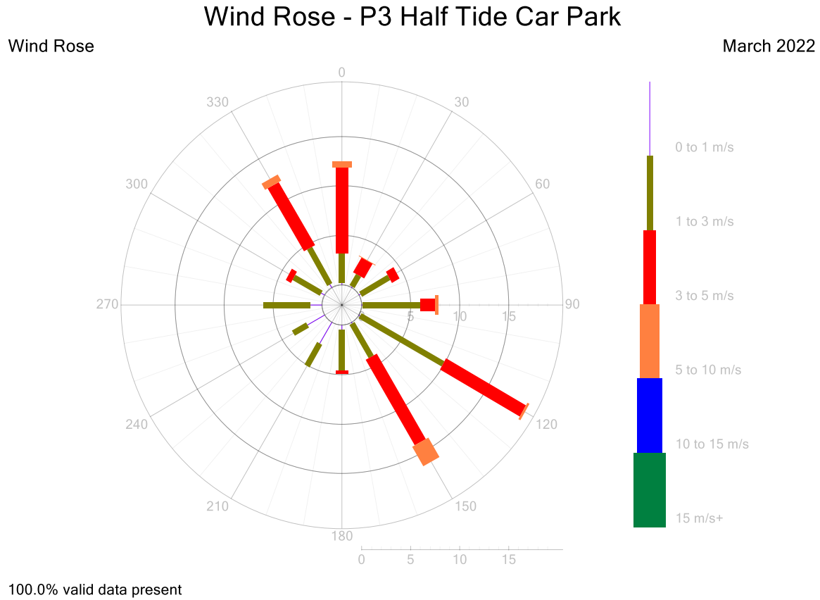
Figure 13: P3 Wind Rose 5-Minute Data for March 2022
