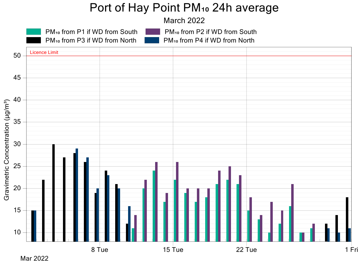
Figure 4: Port of Hay Point PM 10 24-Hour Average Data Compared to the Licence Limit for March 2022
