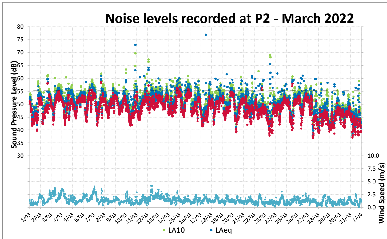
Figure 8: Noise Levels Recorded at P2 for March 2022
