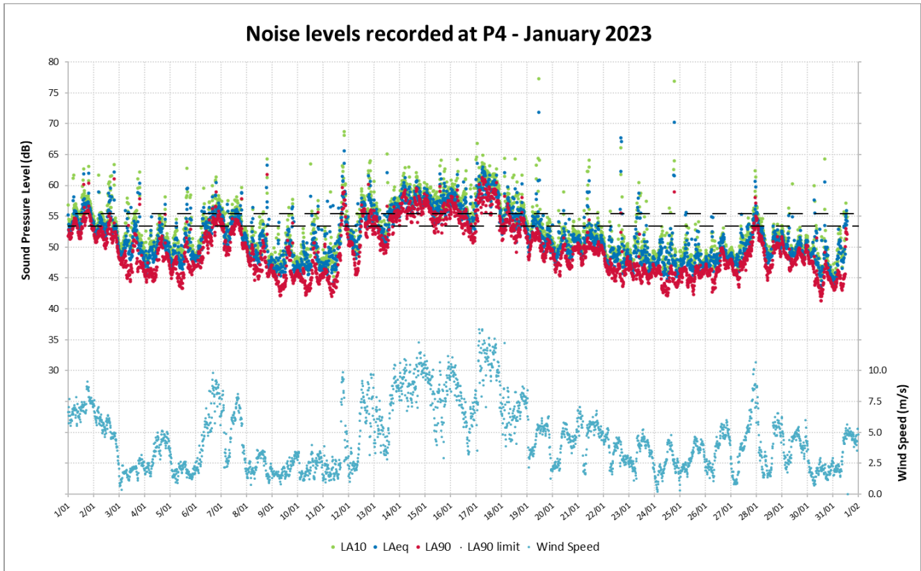
Figure 10: Noise Levels Recorded at P4 for January 2023
