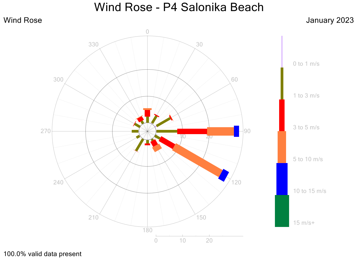
Figure 14: P4 Wind Rose 5-Minute Data for January 2023
