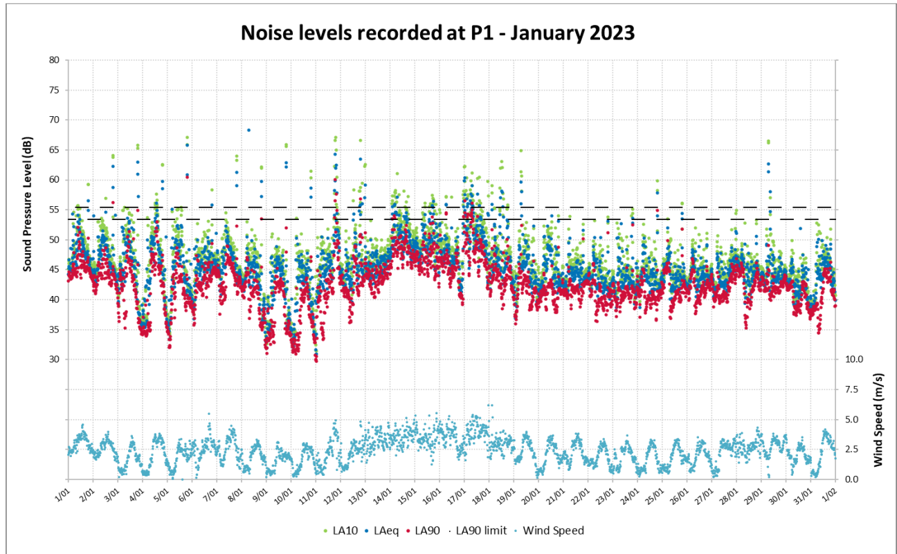
Figure 7: Noise Levels Recorded at P1 for January 2023
