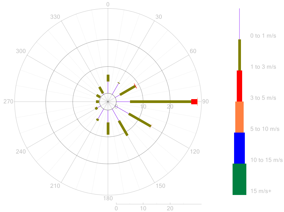
Figure 12: P2 Wind Rose 5-Minute Data for January 2023
