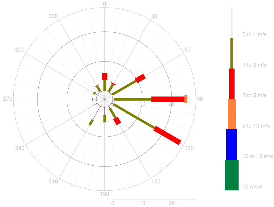
Figure 11: P1 Wind Rose 5-Minute Data for January 2023
