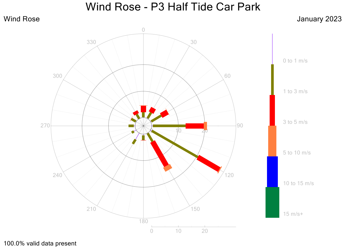
Figure 13: P3 Wind Rose 5-Minute Data for January 2023
