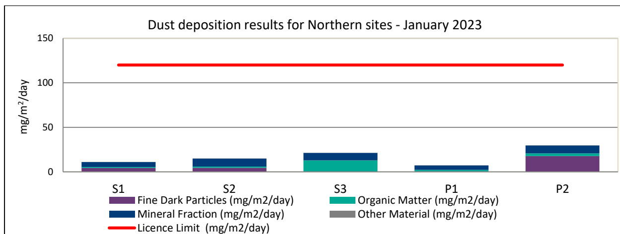
Figure 5: Dust Deposition Results for Northern Sites, January 2023
