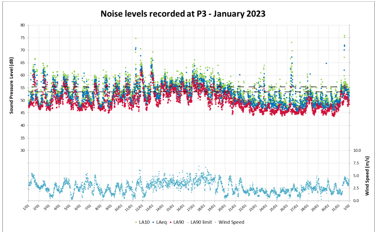
Figure 9: Noise Levels Recorded at P3 for January 2023
