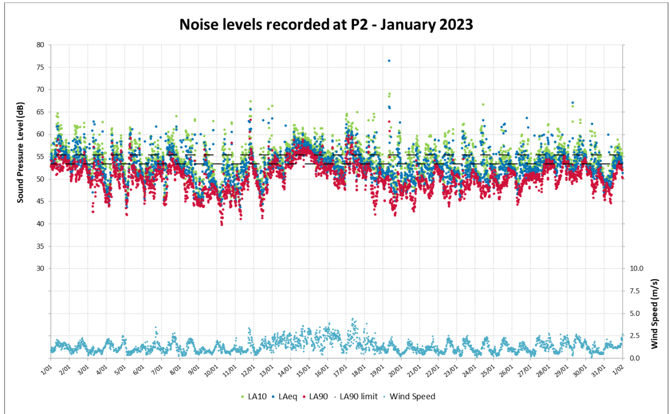
Figure 8: Noise Levels Recorded at P2 for January 2023
