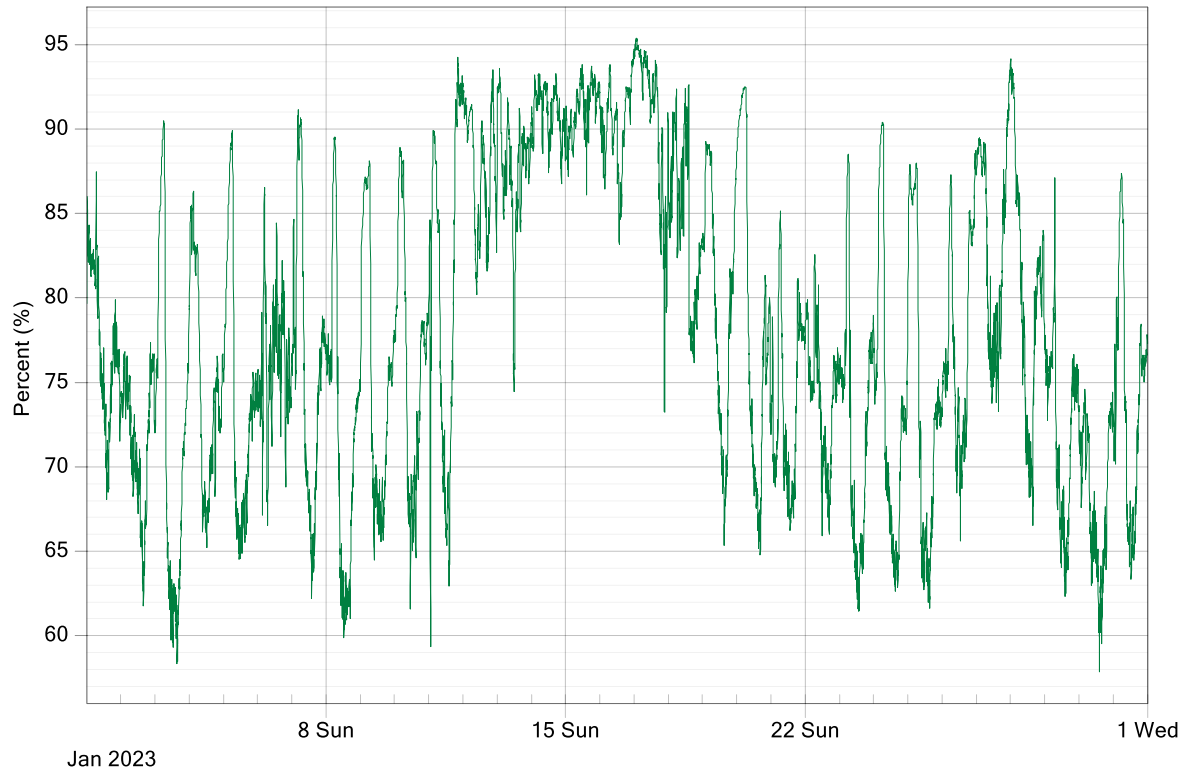
Figure 16: Port of Hay Point RH 5-Minute Averages Data for January 2023
