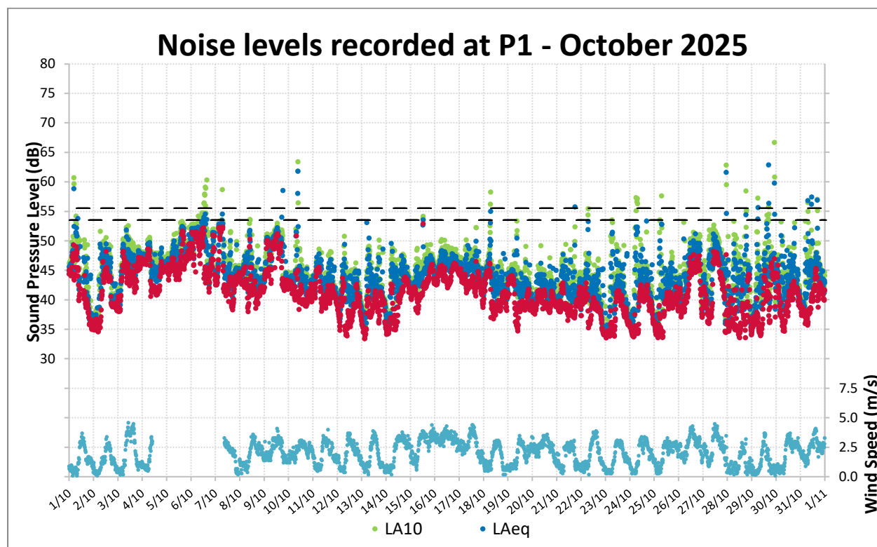
Figure 7: Noise Levels Recorded at P1 for October 2025
