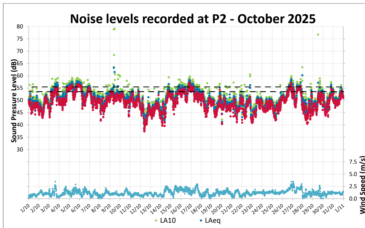
Figure 8: Noise Levels Recorded at P2 for October 2025
