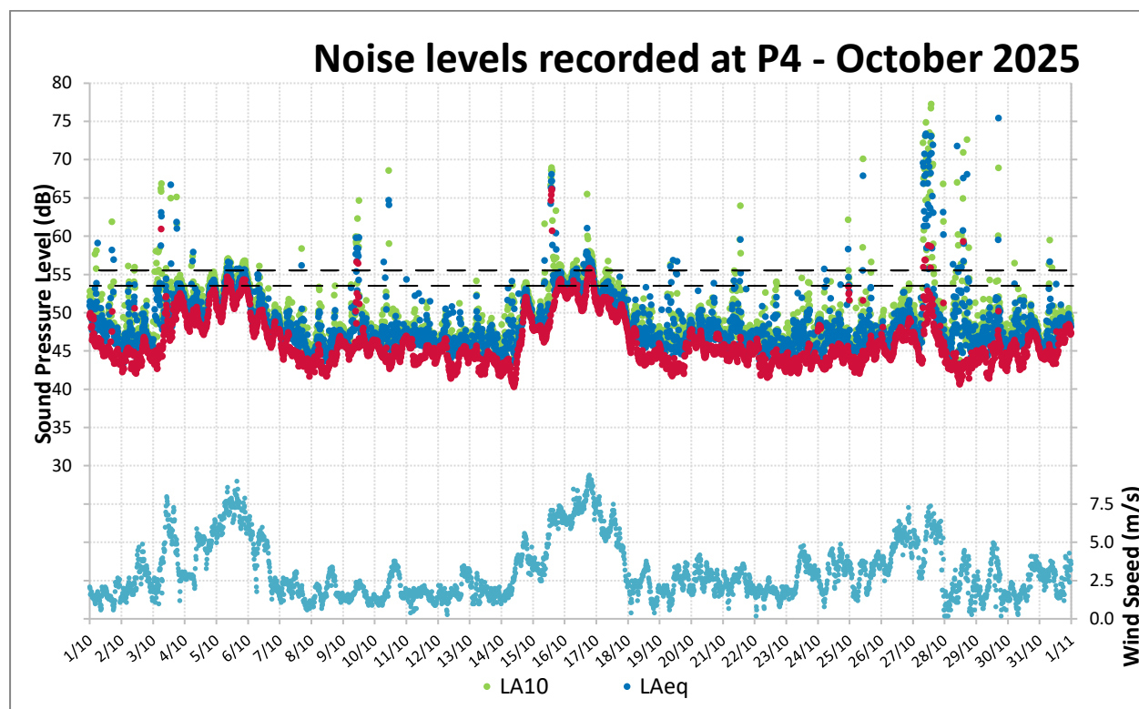
Figure 10: Noise Levels Recorded at P4 for October 2025
