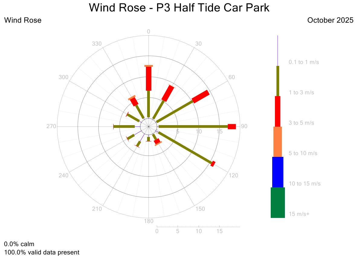
Figure 13: P3 Wind Rose 5-Minute Data for October 2025
