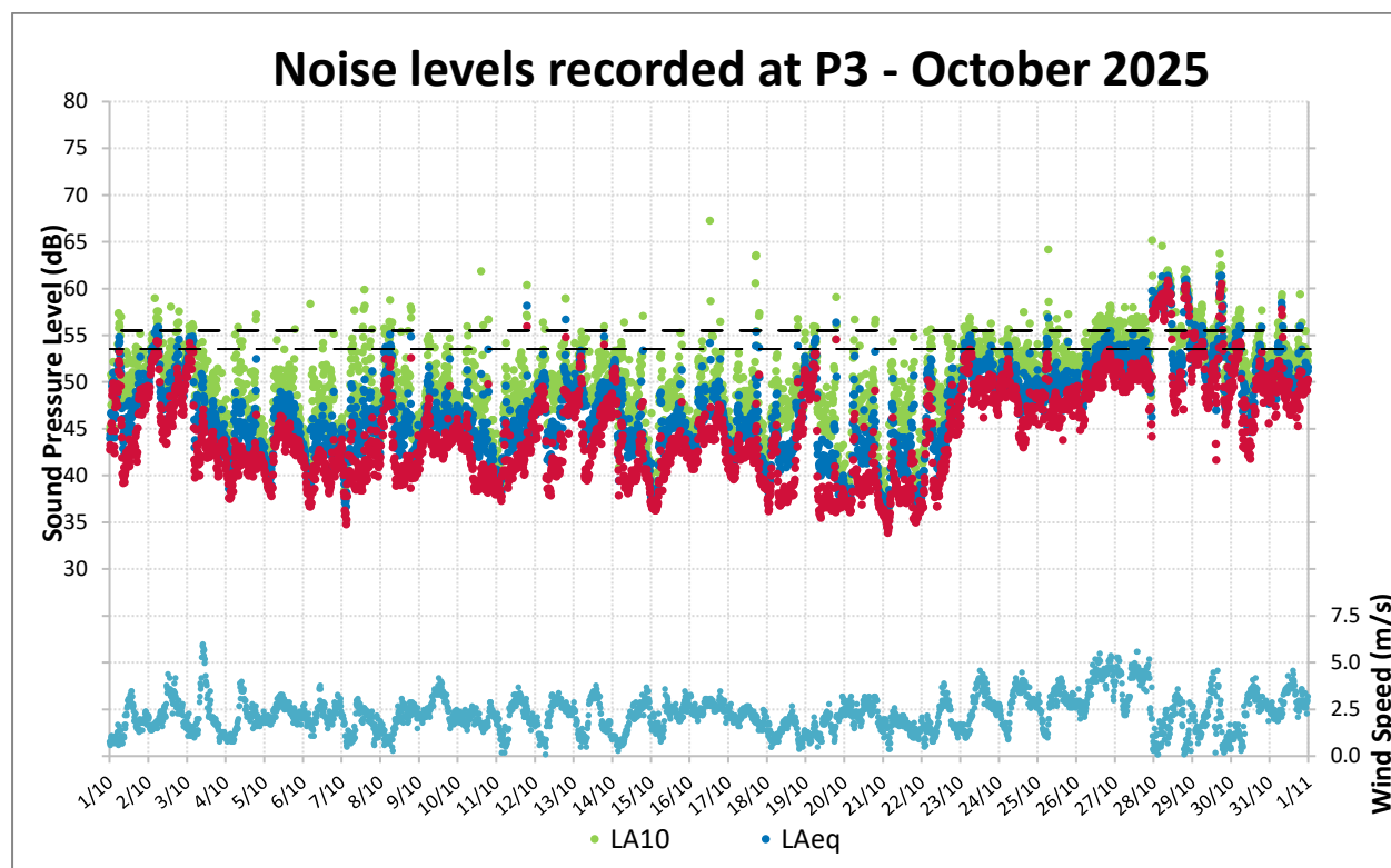
Figure 9: Noise Levels Recorded at P3 for October 2025
