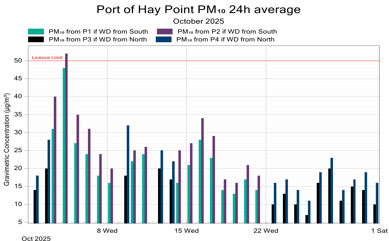
Figure 4: Port of Hay Point PM 10 24-Hour Average Data Compared to the Licence Limit for October 2025 5
