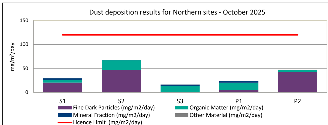
Figure 5: Dust Deposition Results for Northern Sites, October 2025
