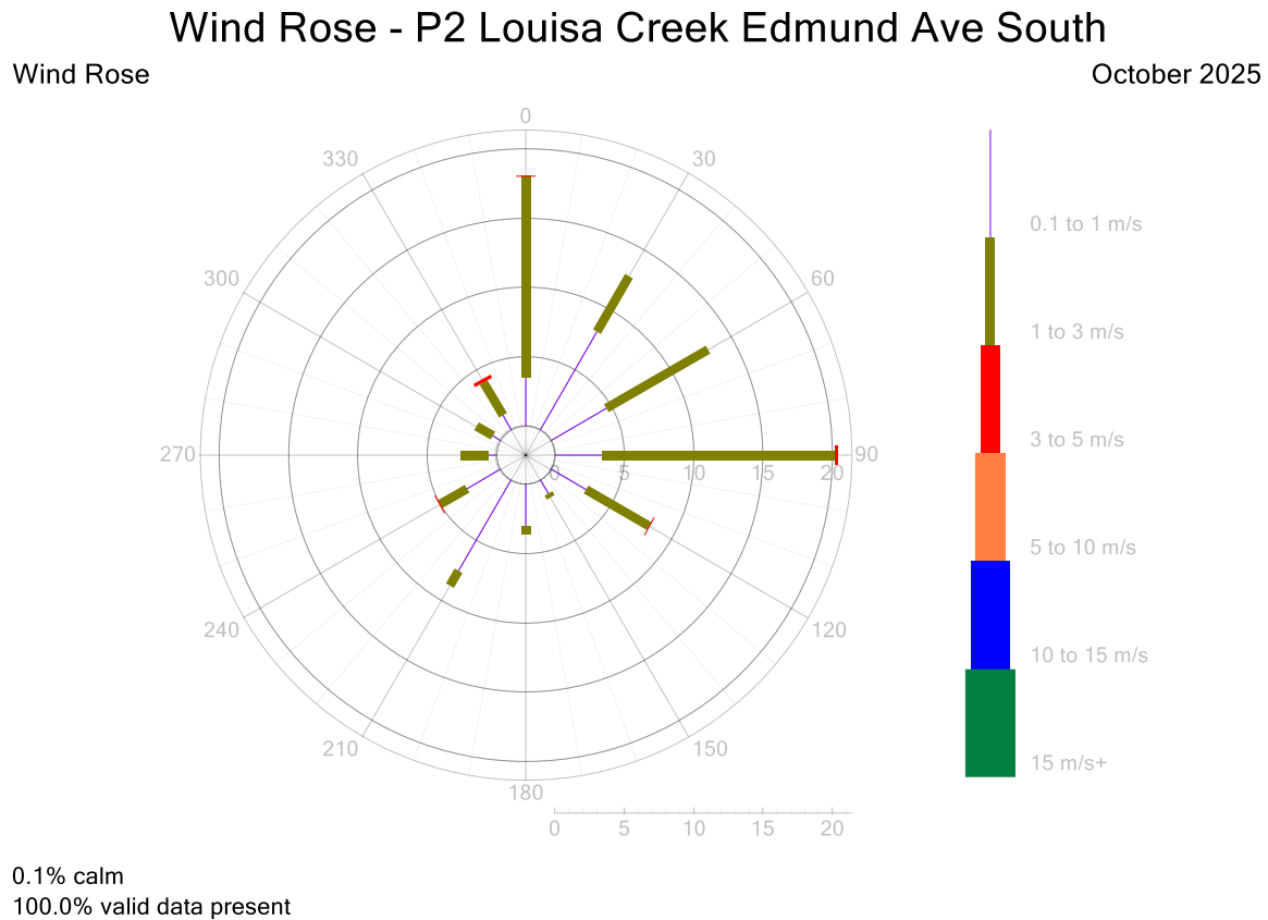
Figure 12: P2 Wind Rose 5-Minute Data for October 2025
