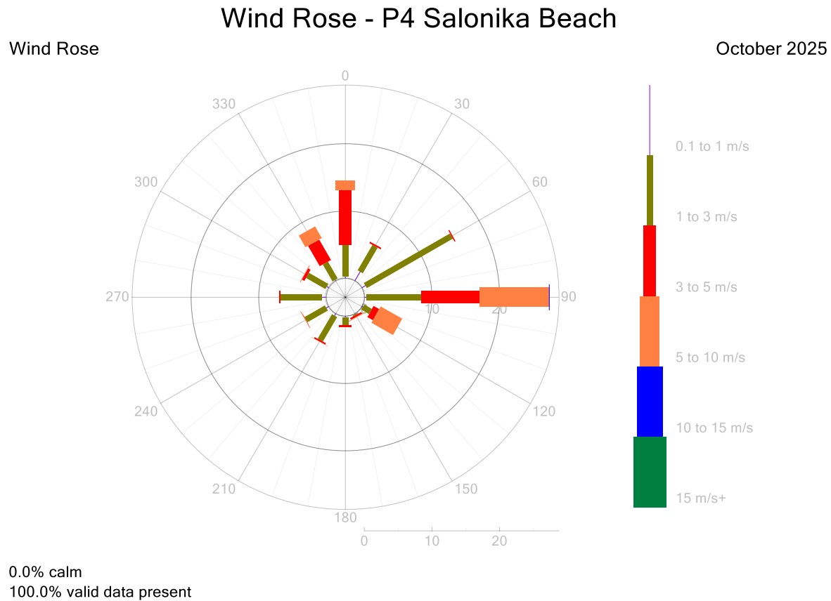
Figure 14: P4 Wind Rose 5-Minute Data for October 2025
