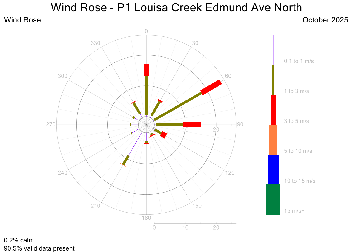
Figure 11: P1 Wind Rose 5-Minute Data for October 2025
