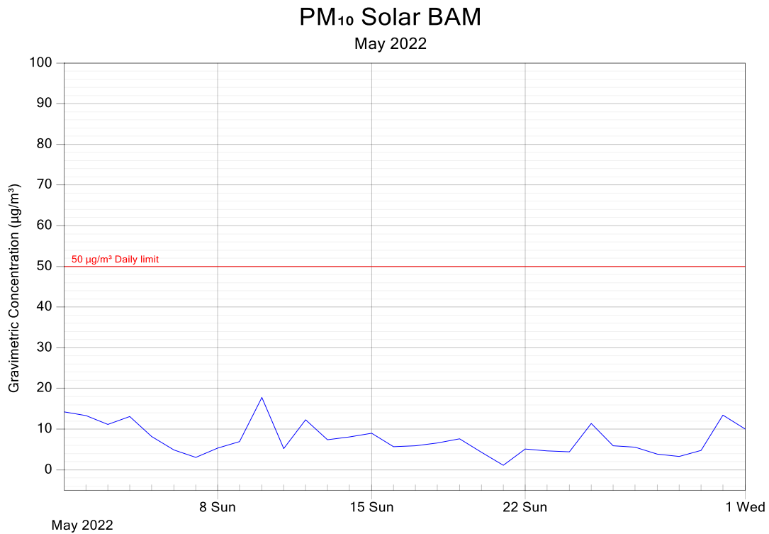
Figure 2: PM 10 for McEwens Beach station 24-hour Averages – May 2022
