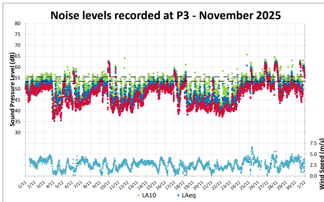
Figure 9: Noise Levels Recorded at P3 for November 2025
