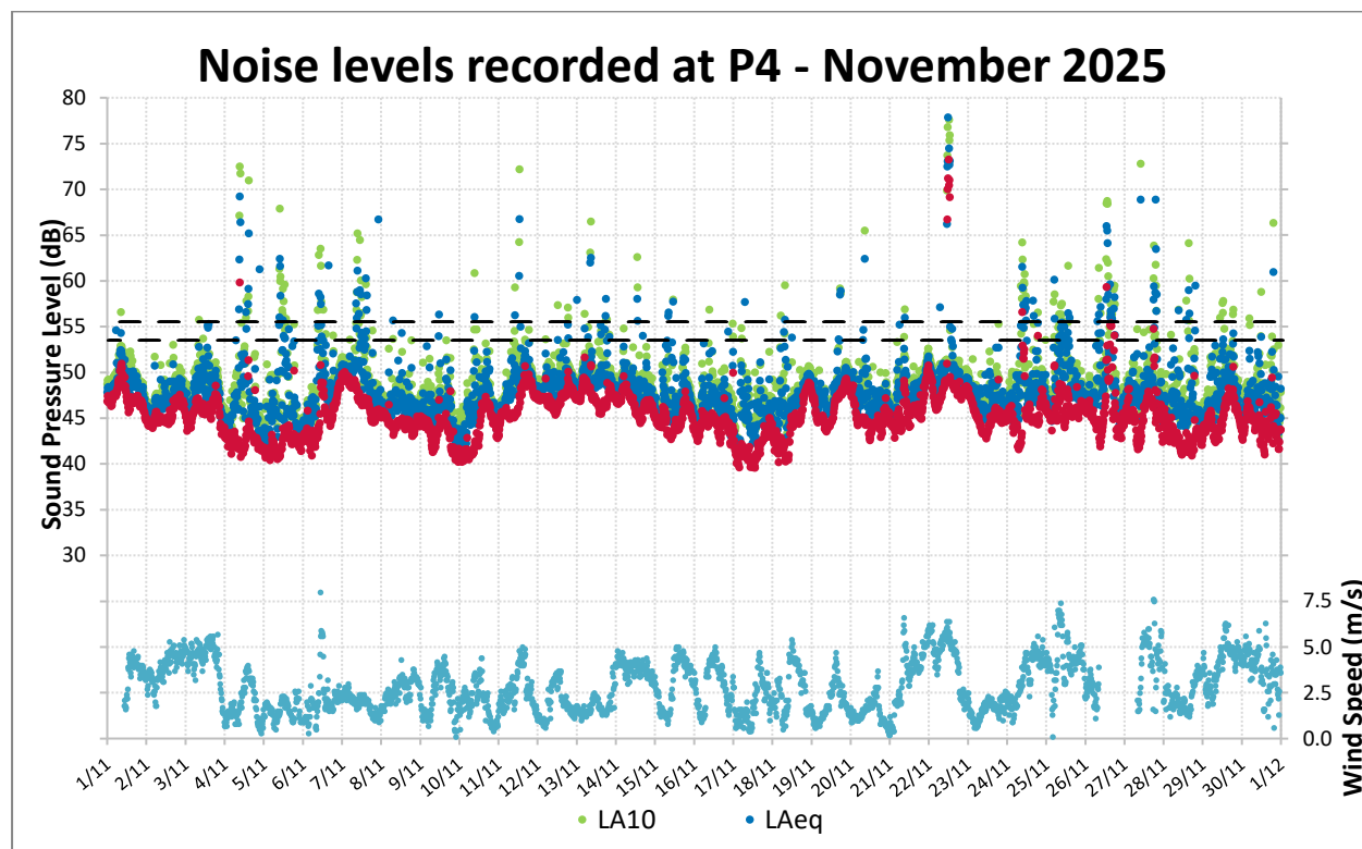
Figure 10: Noise Levels Recorded at P4 for November 2025
