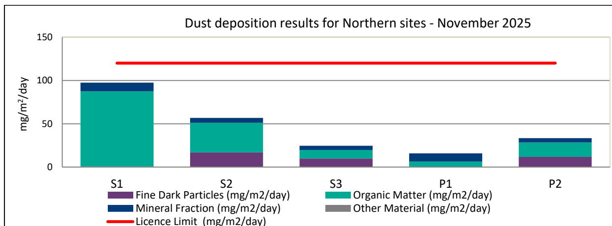
Figure 5: Dust Deposition Results for Northern Sites, November 2025
