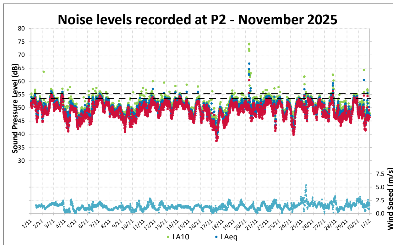
Figure 8: Noise Levels Recorded at P2 for November 2025
