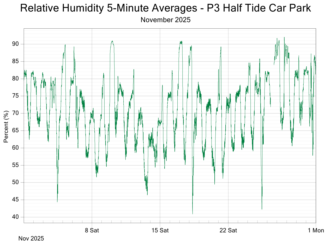
Figure 16: Port of Hay Point RH 5-Minute Averages Data for November 2025
