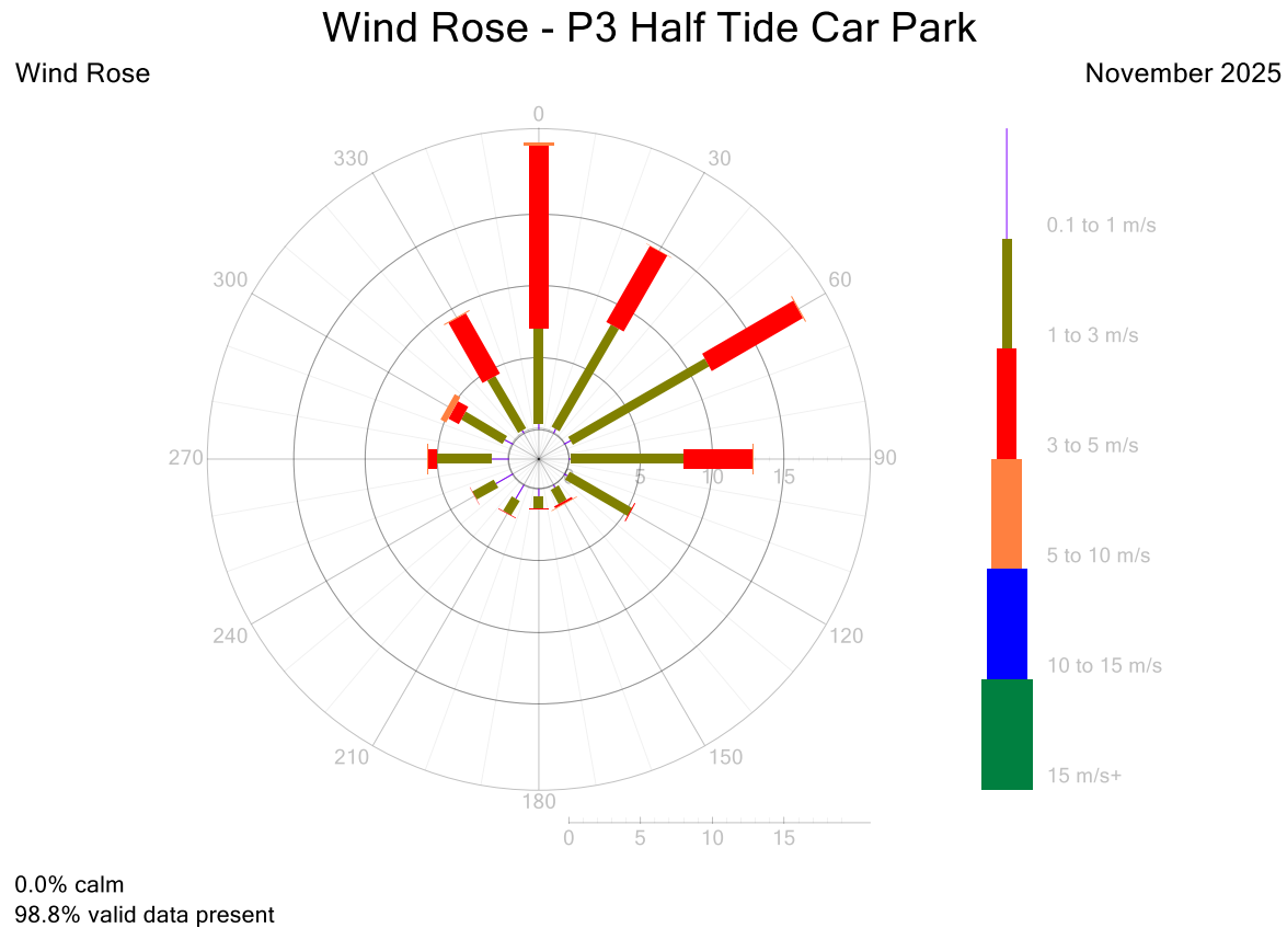
Figure 13: P3 Wind Rose 5-Minute Data for November 2025
