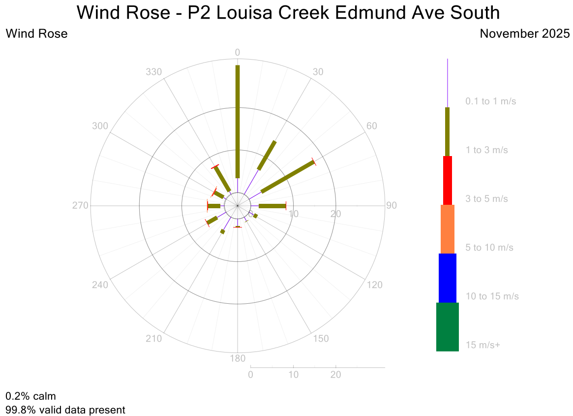
Figure 12: P2 Wind Rose 5-Minute Data for November 2025
