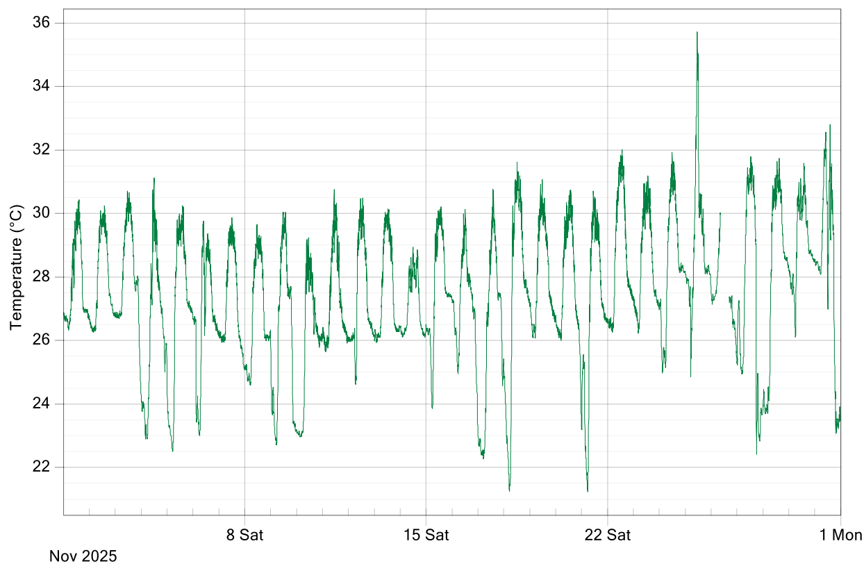
Figure 15: Port of Hay Point AT 5-Minute Averages Data for November 2025
