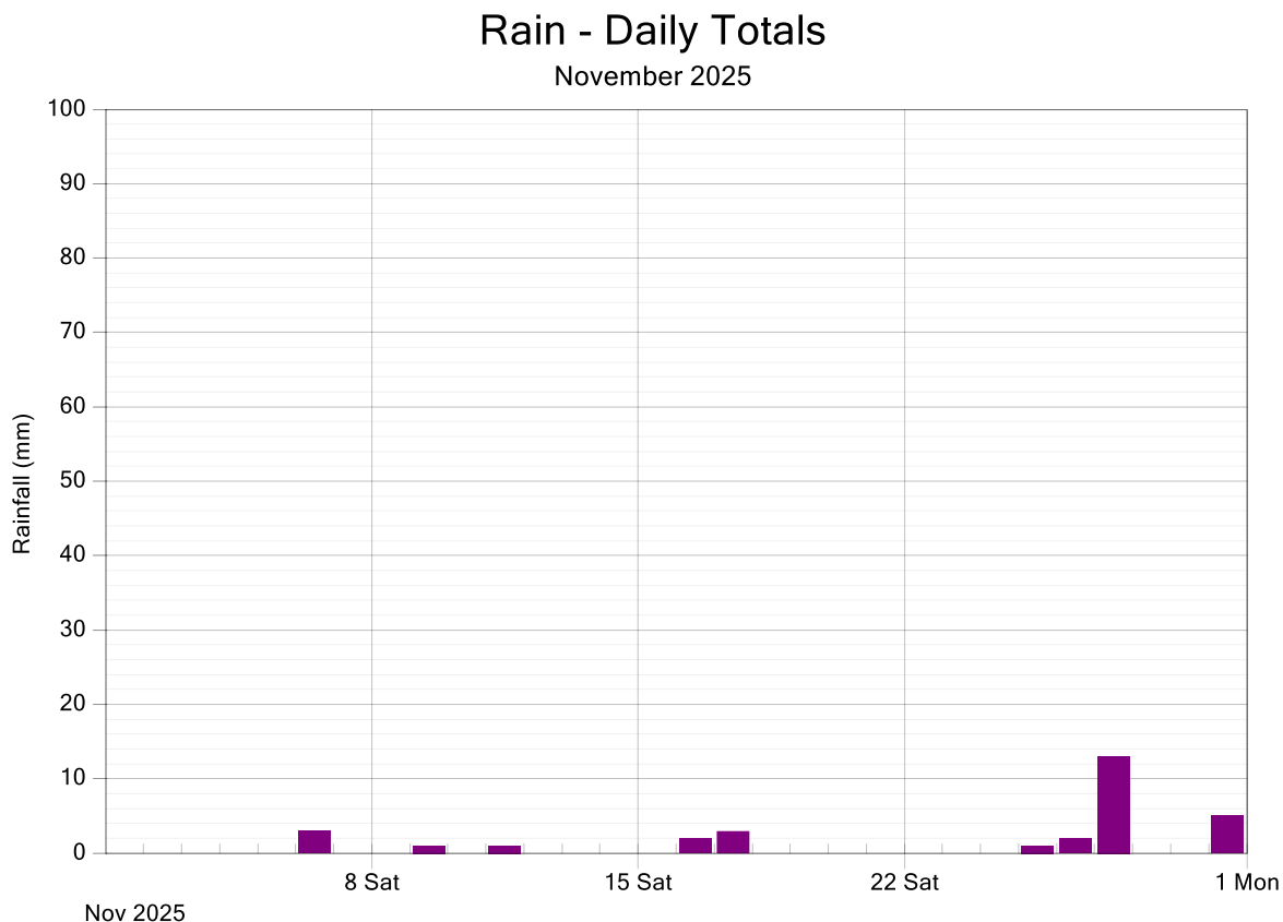
Figure 17: Port of Hay Point Rain Daily Totals for November 2025
