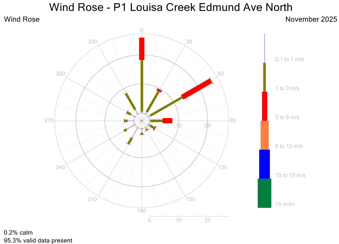
Figure 11: P1 Wind Rose 5-Minute Data for November 2025
