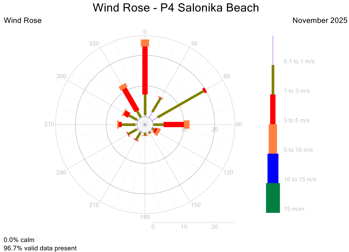
Figure 14: P4 Wind Rose 5-Minute Data for November 2025
