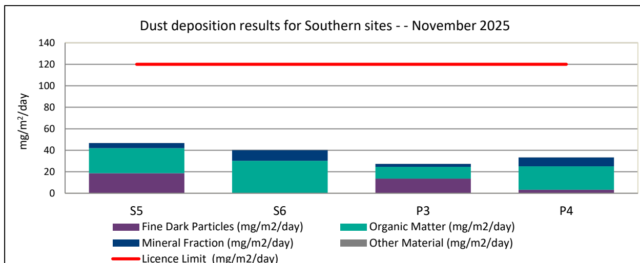
Figure 6: Dust Deposition Results for Southern Sites, November 2025
