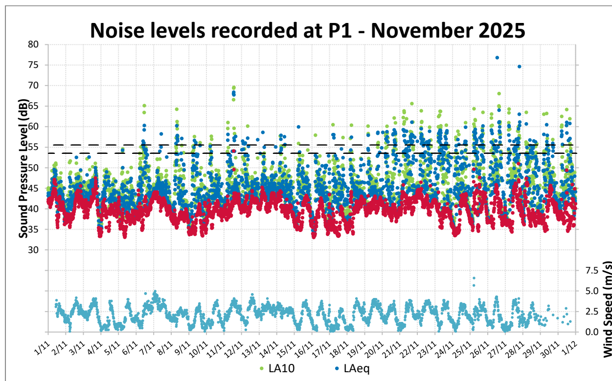
Figure 7: Noise Levels Recorded at P1 for November 2025
